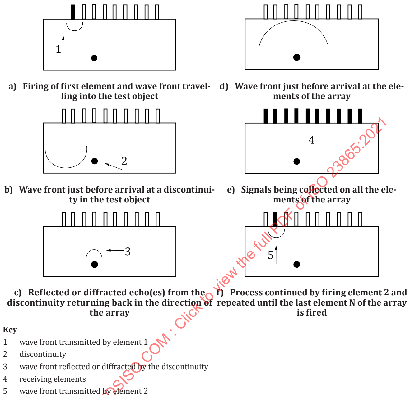
Figure 1 — Typical example of points in time describing the FMC data collection process
