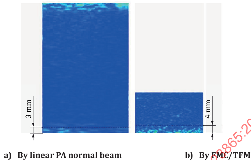
Figure D.3 — Comparison of PAUT and FMC/TFM on early HTHA damage
