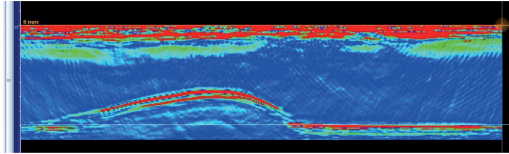
Figure D.6 — FMC/TFM image on a shallow wide internal corrosion
