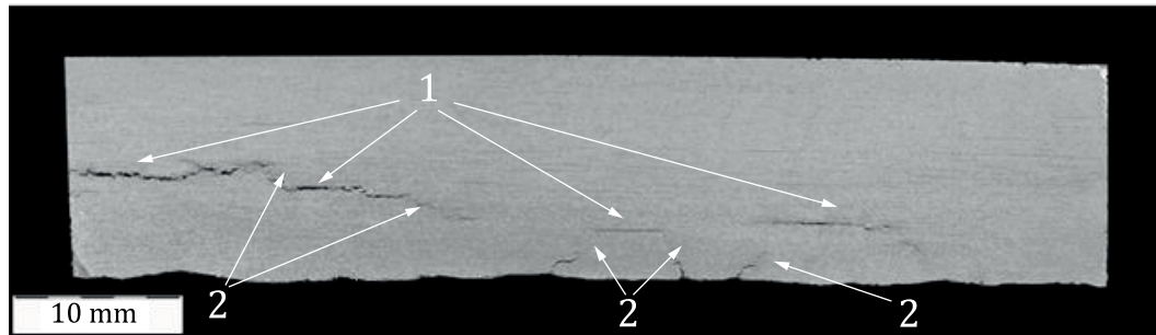
b) Macro section corresponding to the FMC/TFM image
