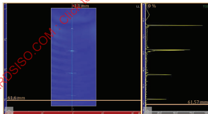
Figure D.1 — Sensitivity correction (Frequency 15 MHz - LL imaging path)
