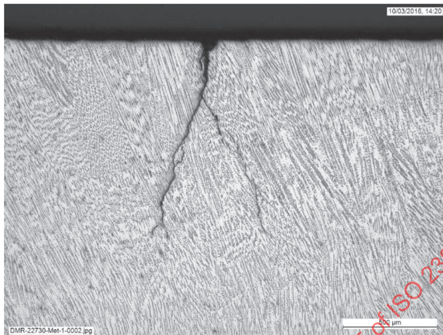
Figure D.8 — Micrographs of a SCC in stainless steel weld overlay cladding
