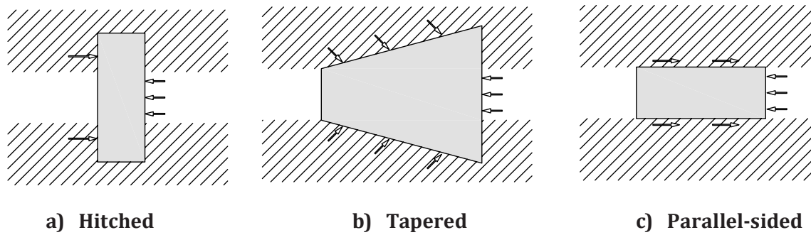
Figure 1 — Shapes of high-pressure bulkheads
