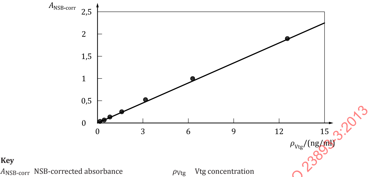
Figure A.2 — Linear curve fit of fathead minnow Vtg standard curve in sandwich ELISA
