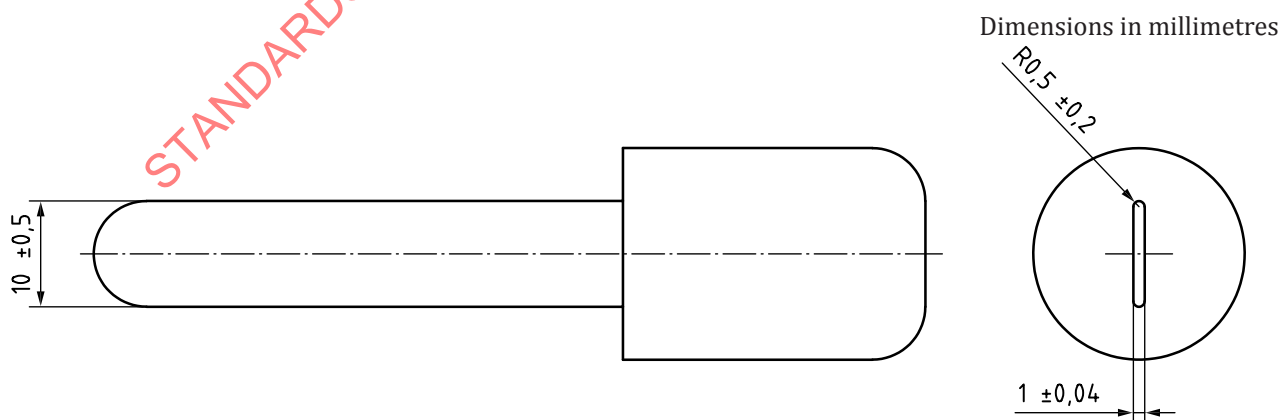
Figure 2 — Metal mandrel
