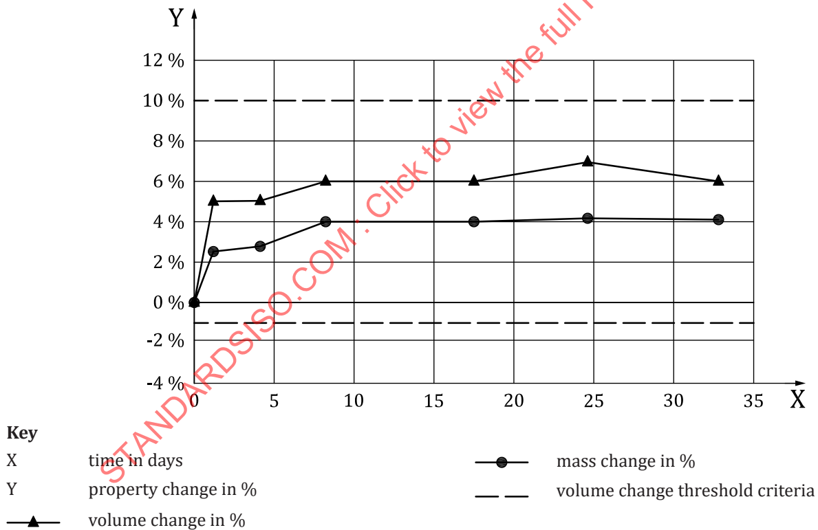
Figure A.9 — Example T_1 volume and mass property change percentages
