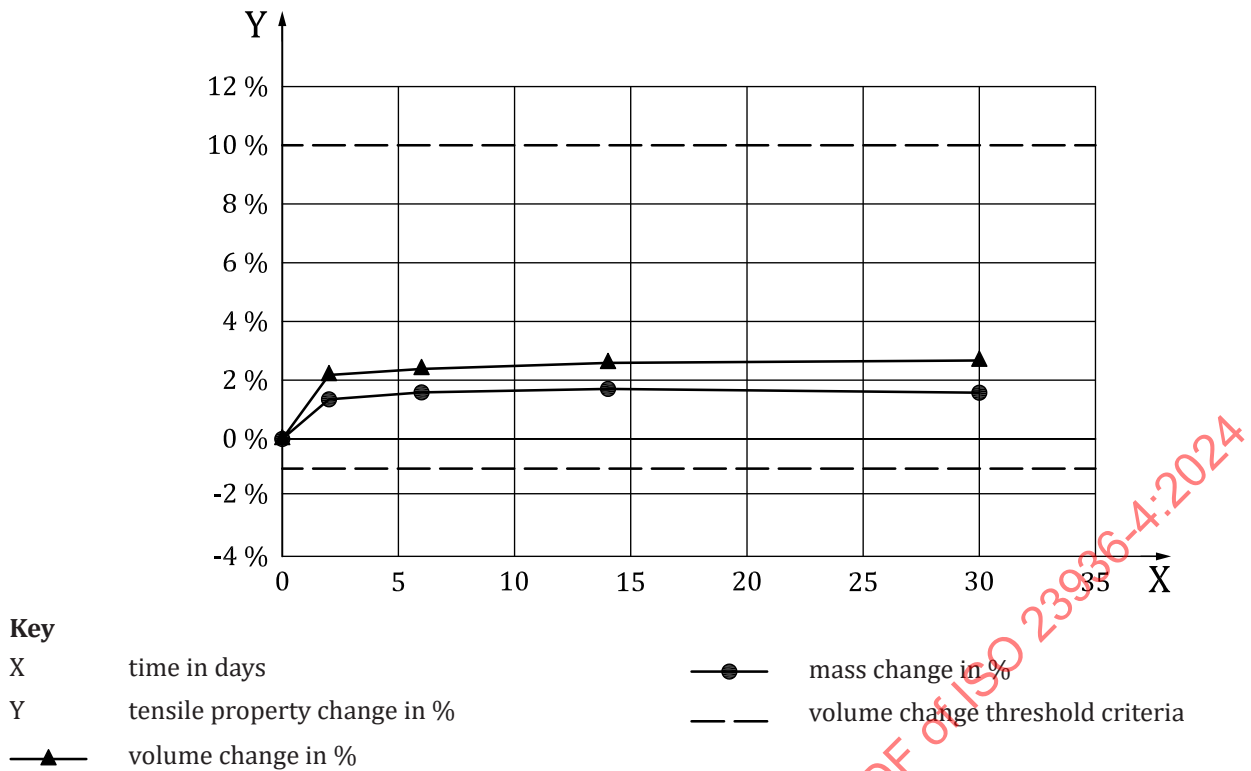
Figure A.5 — Volume and mass property change percentages
