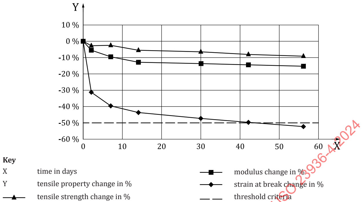
Figure A.8 — Example T_1 tensile property change percentages using 2 day baseline data
