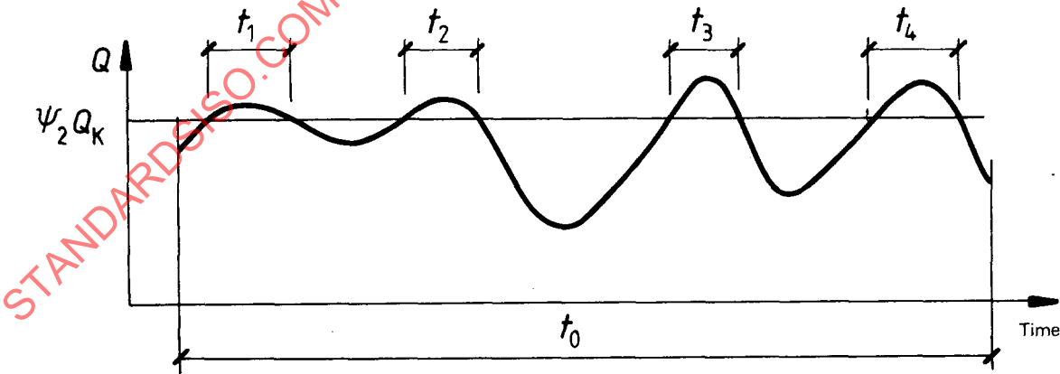
Figure 5 — Quasi-permanent values
