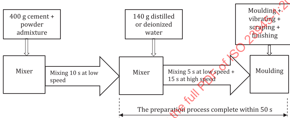
Figure A.1 — Schematic diagram of cement paste preparation with powdery flash setting accelerating admixture
