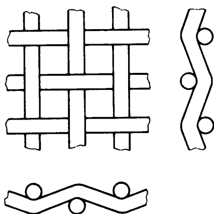
FIGURE 1 — Plain weave
