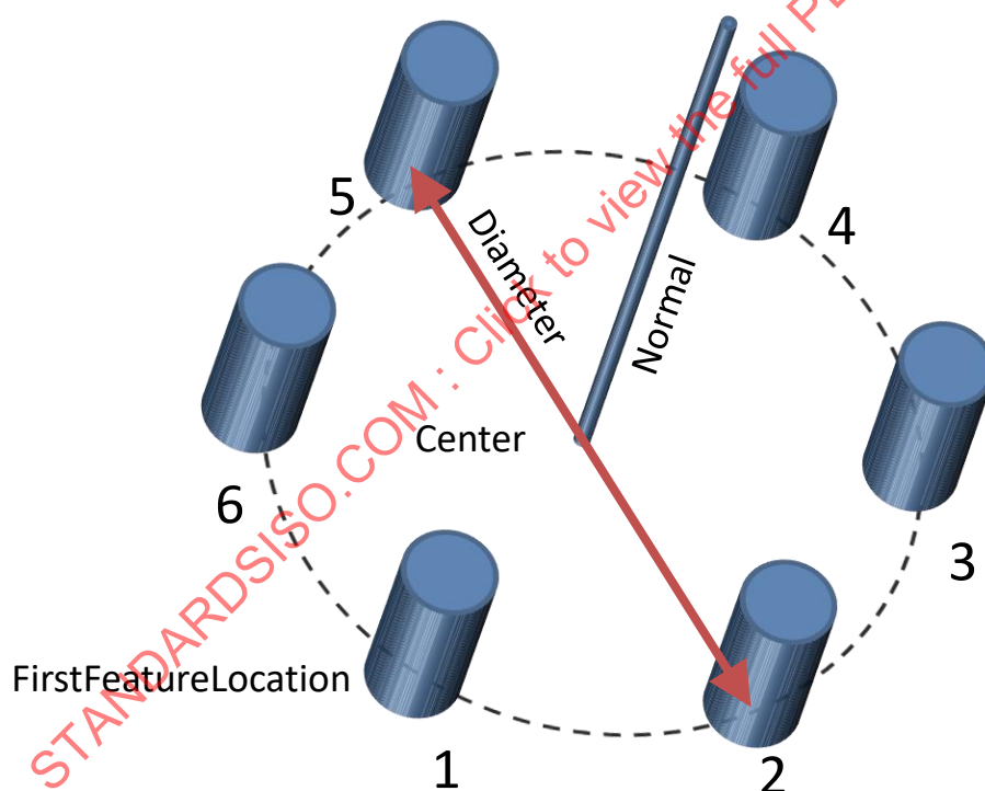
Figure 40 – PatternFeatureCircle with FeatureDirection omitted
