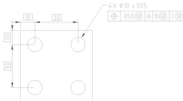
Figure 7 – A plate with four holes and GD&amp;T
