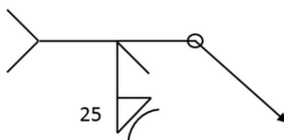
Figure 23 – Compound Weld
