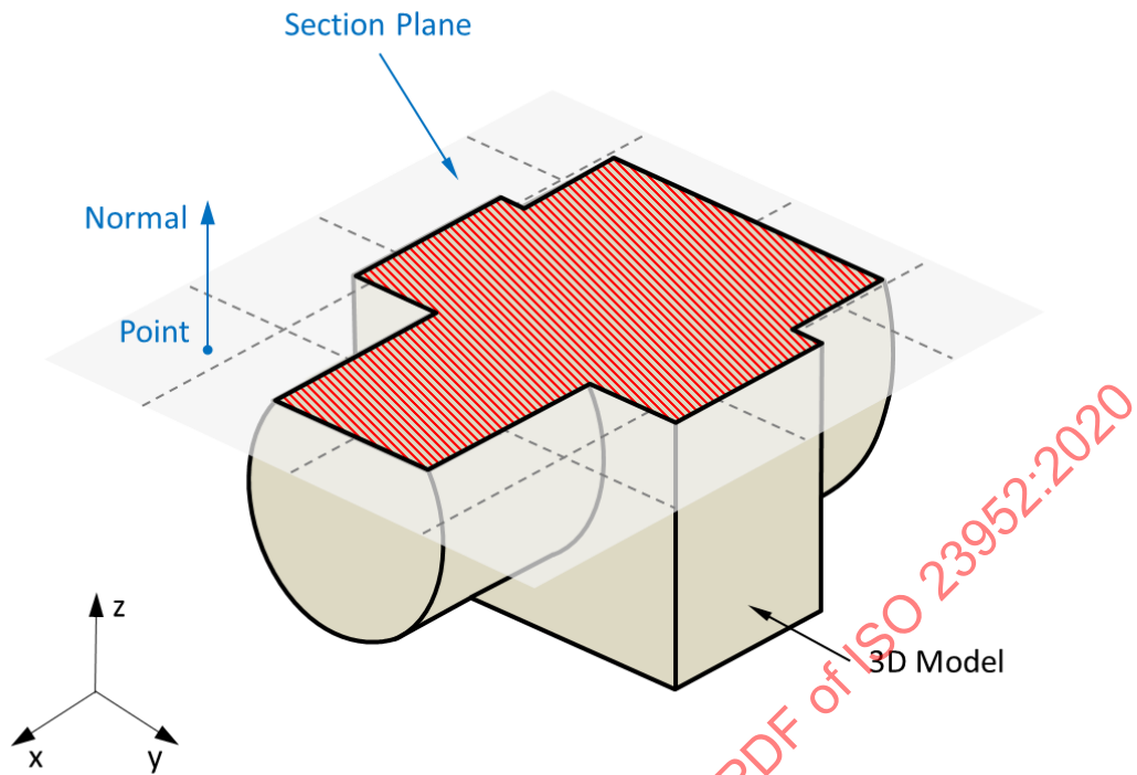
Figure 201 – Zone Section with one section plane
