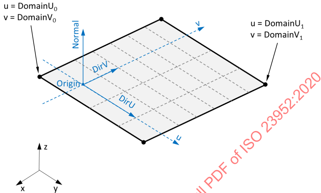
Figure 111 – Plane
