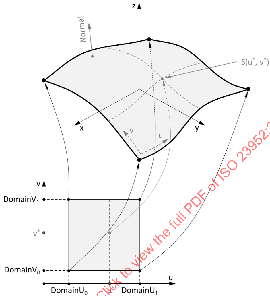
Figure 108 – Parametric Surface
