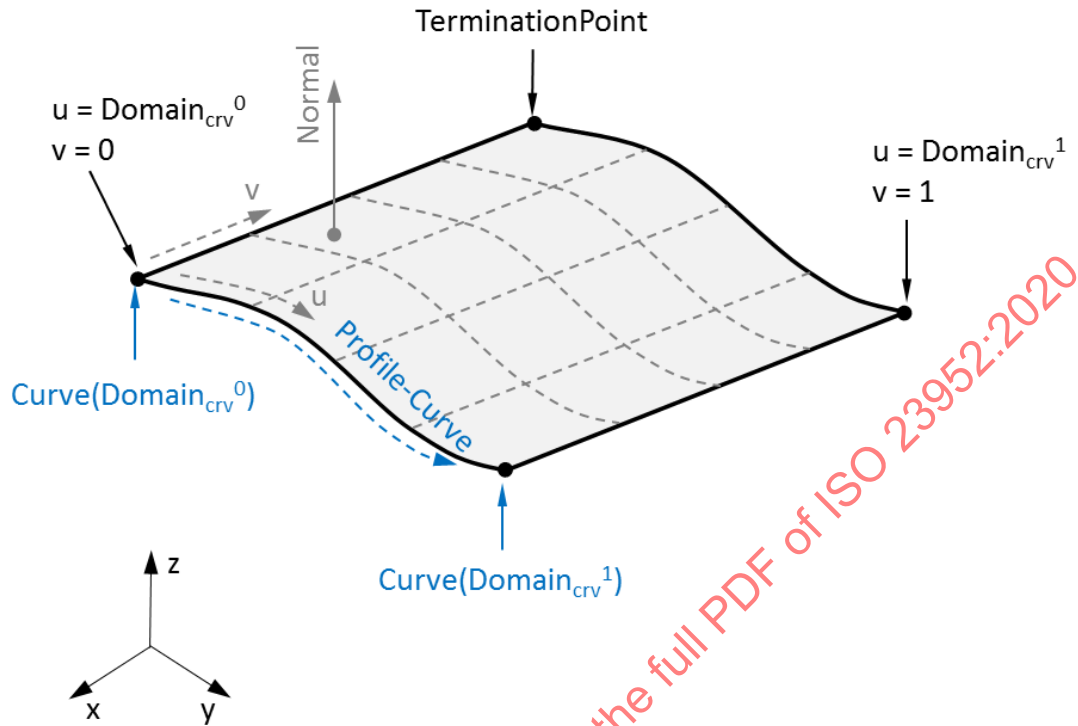
Figure 125 – Extrude Surface
