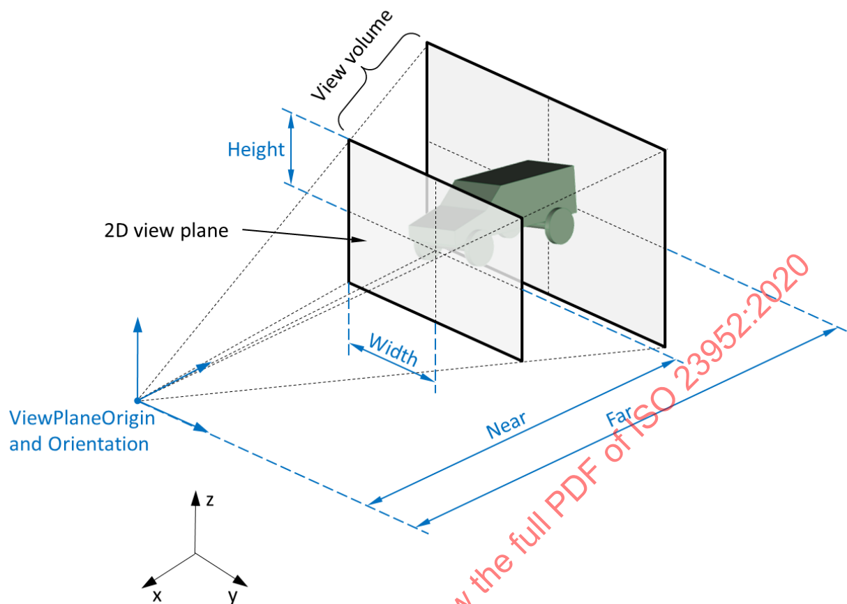
Figure 211 – Perspective Camera
