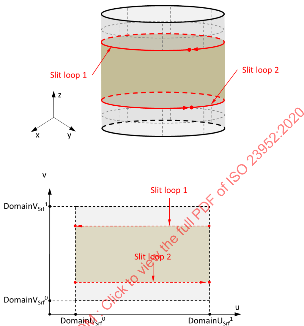
Figure 152 – Slit Loop
