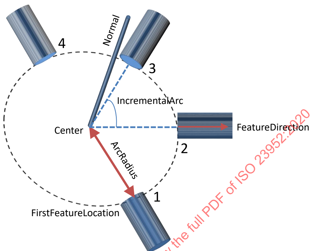
Figure 42 – PatternFeatureCircularArc
