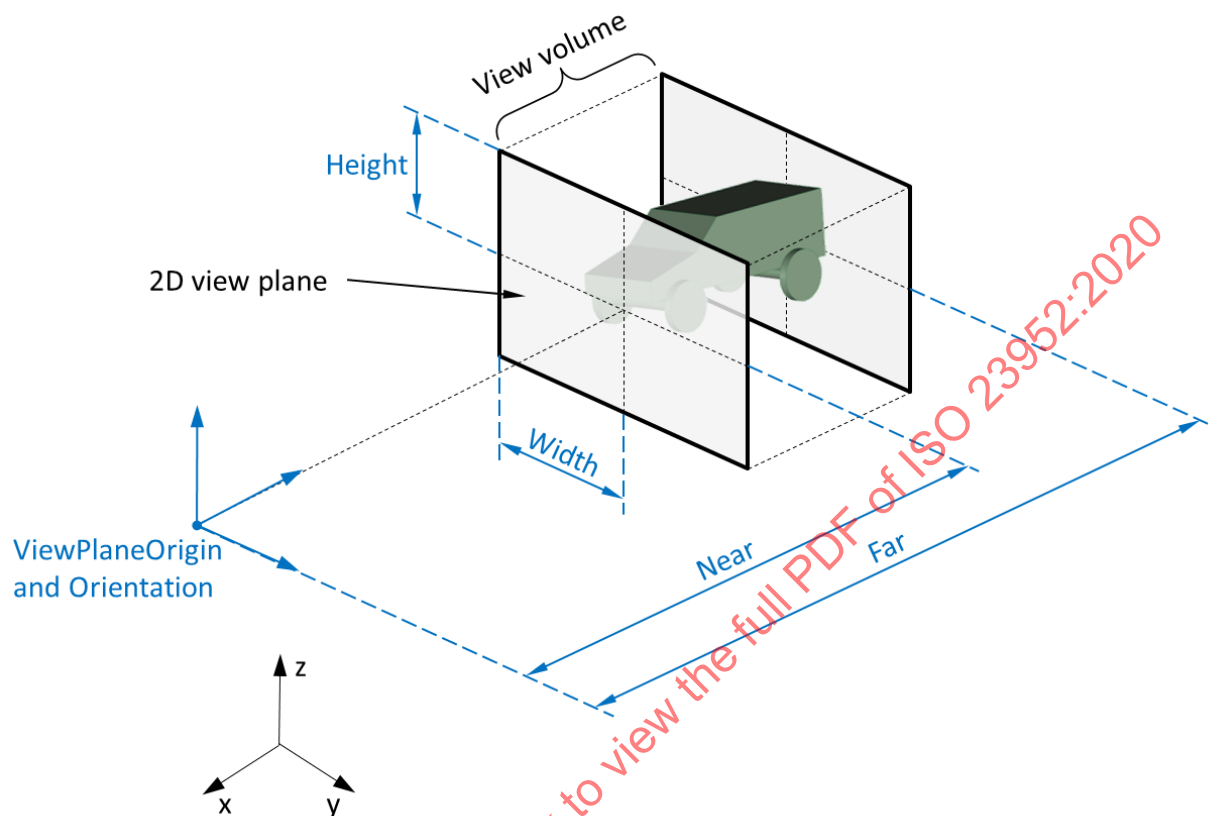
Figure 197 – Saved view
