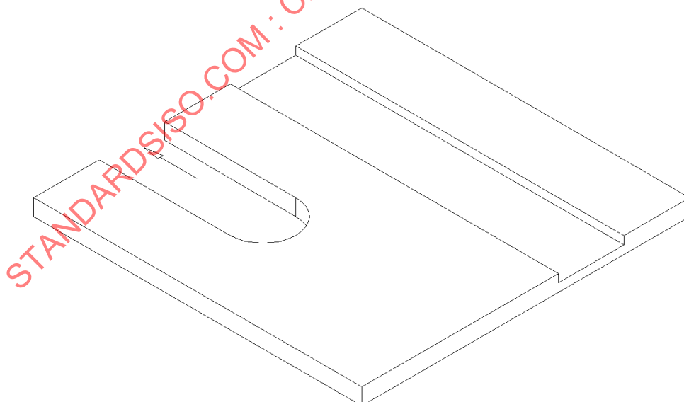
Figure 29 – Opposite planes features with open ends
