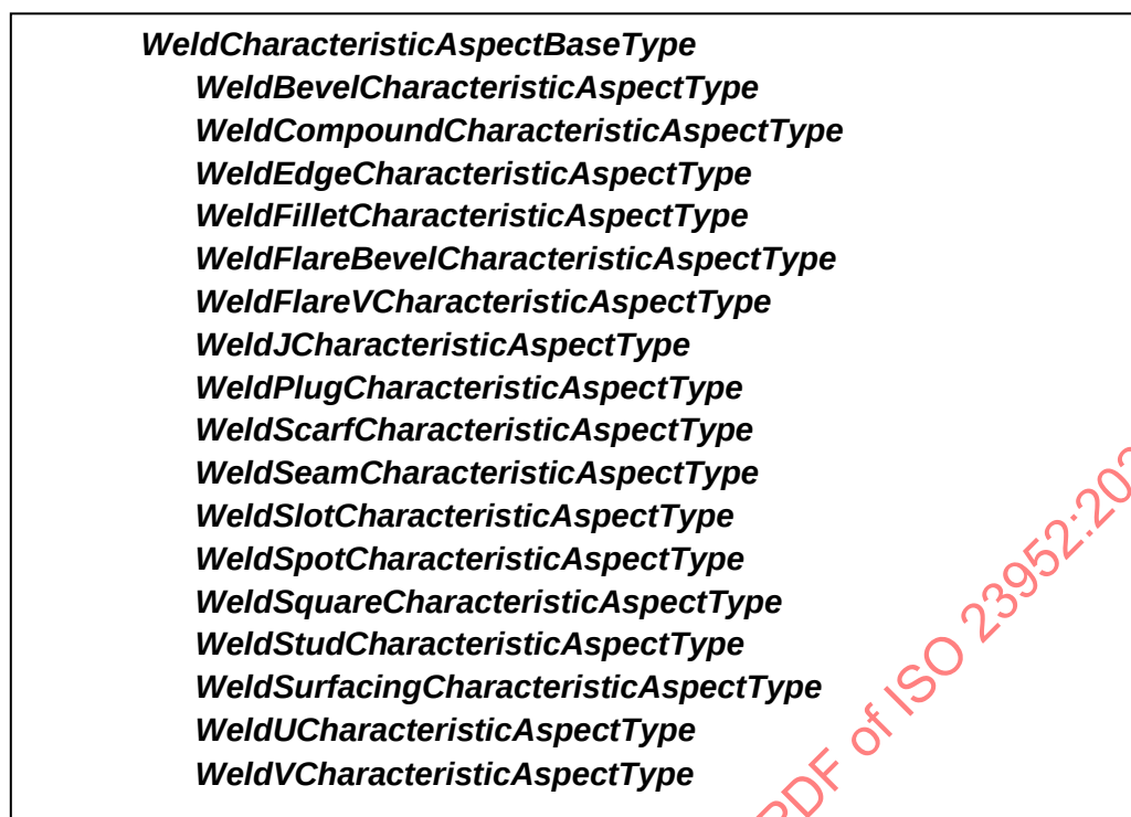
Figure 49 – Characteristic types
