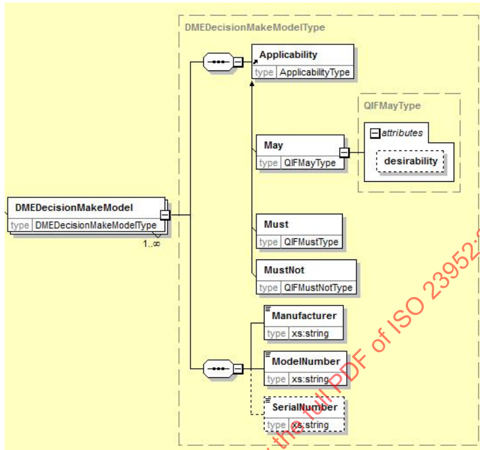
Figure 232 – DMEDecisionMakeModel element
