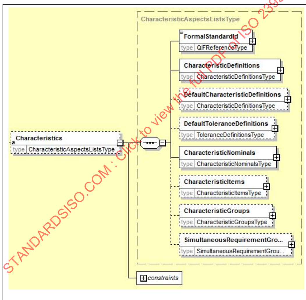
Figure 48 – Characteristics element
