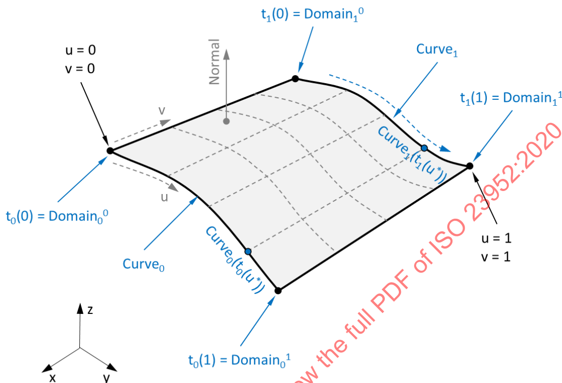
Figure 127 – Ruled Surface
