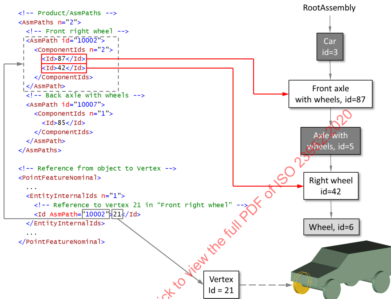
Figure 170 – Reference of a part entity within an assembly
