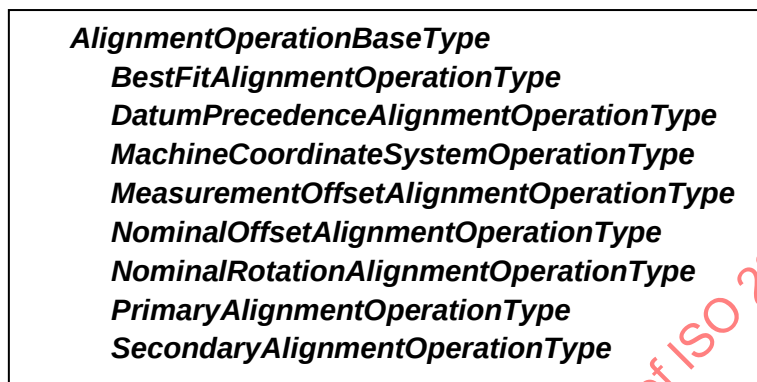
Figure 56 – Alignment operations
