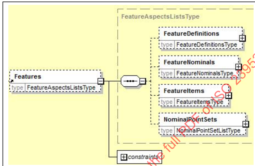
Figure 51 – Features element
