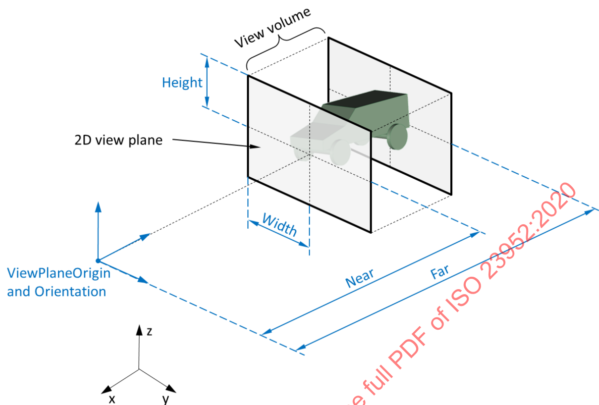
Figure 210 – Orthographic Camera
