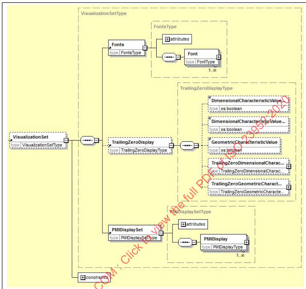
Figure 76 – VisualizationSet element
