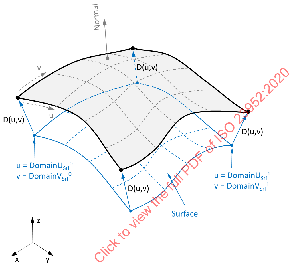
Figure 137 – Offset Surface
