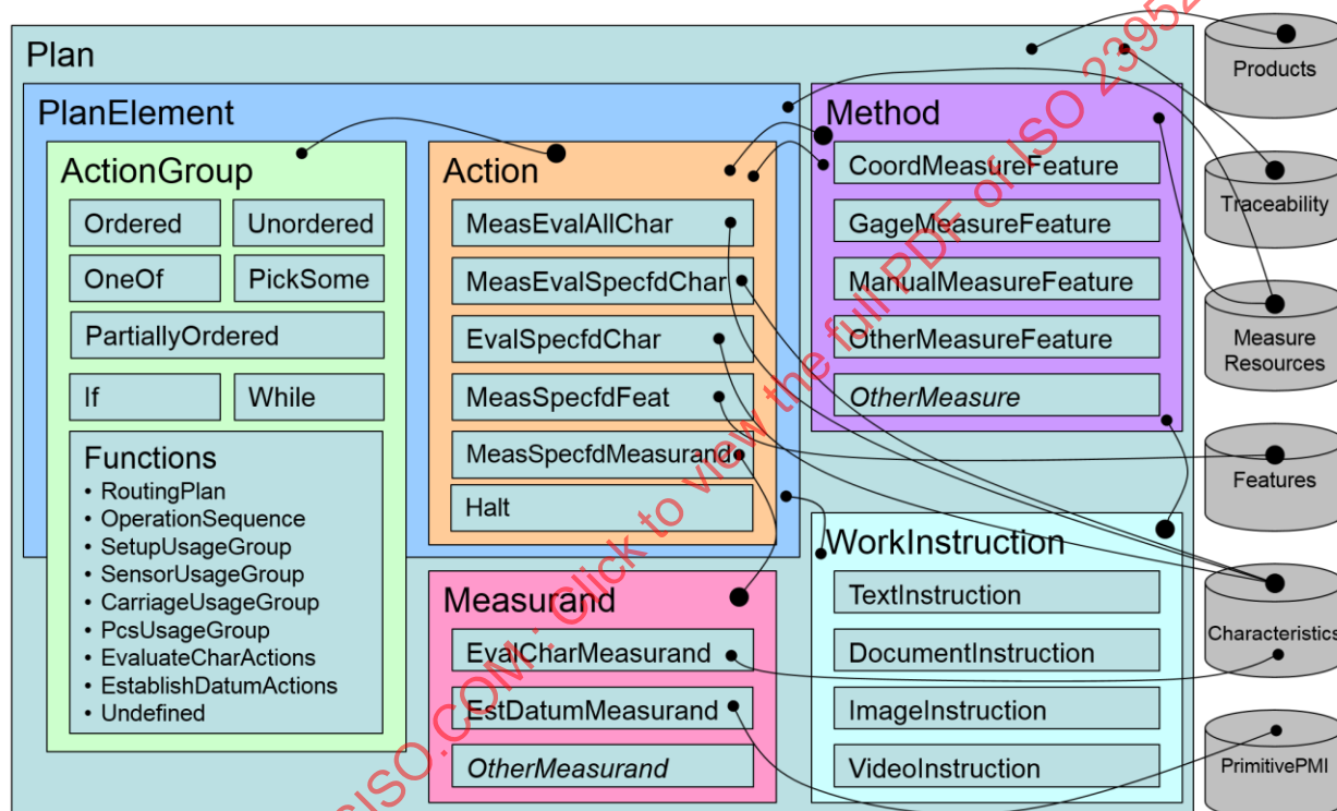
Figure 216 – QIF Plans Major Elements with Simplified Relations
