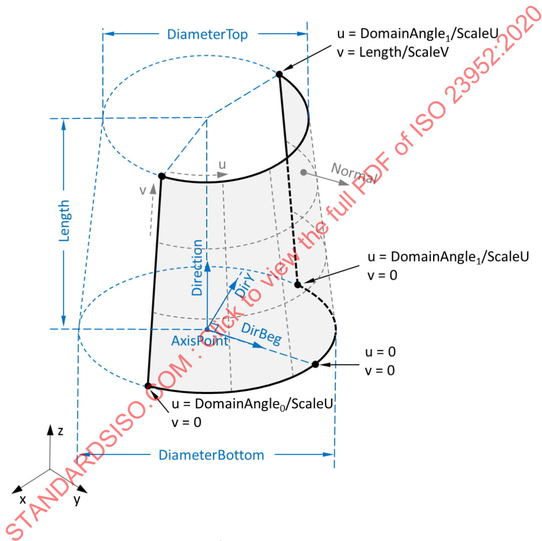
Figure 116 – Cone
