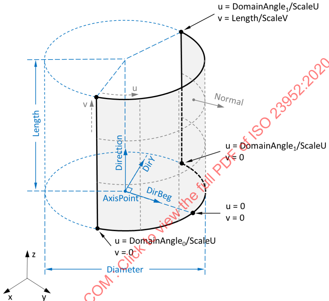
Figure 113 – Cylinder
