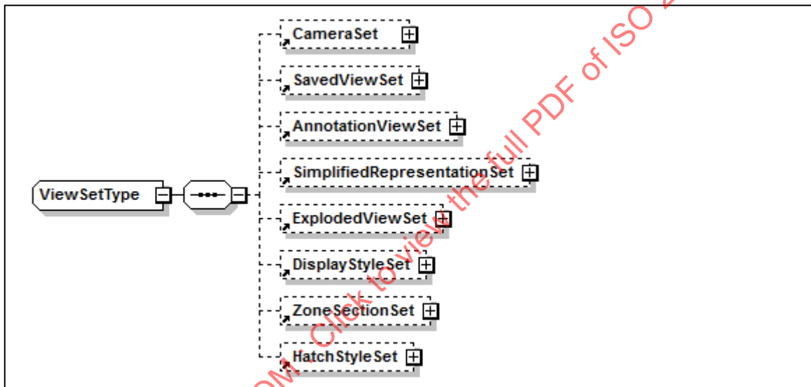
Figure 77 – ViewSetType
