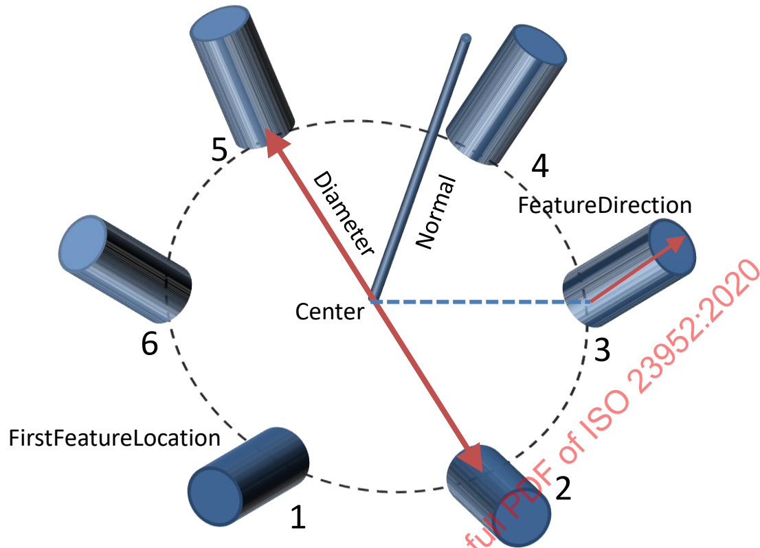
Figure 41 – PatternFeatureCircle with FeatureDirection
