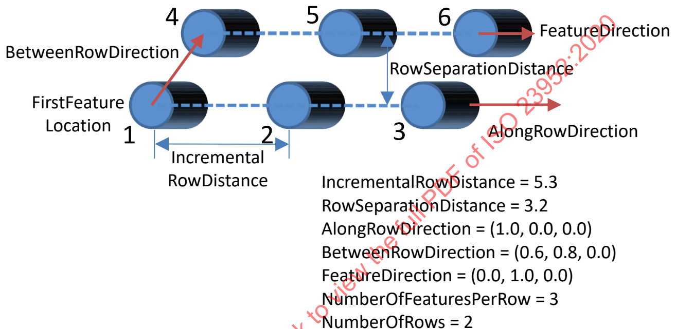
Figure 44 – PatternFeatureParallelogram
