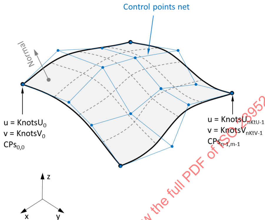
Figure 135 – NURBS Surface
