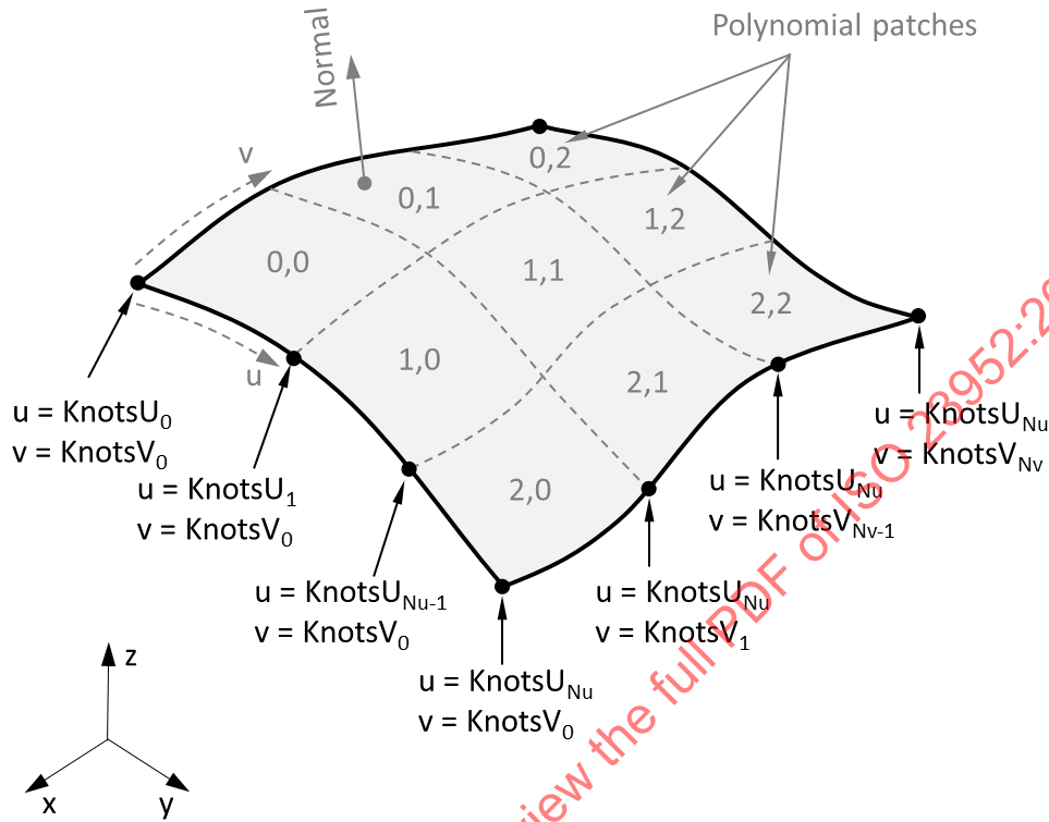
Figure 133 – Spline Surface
