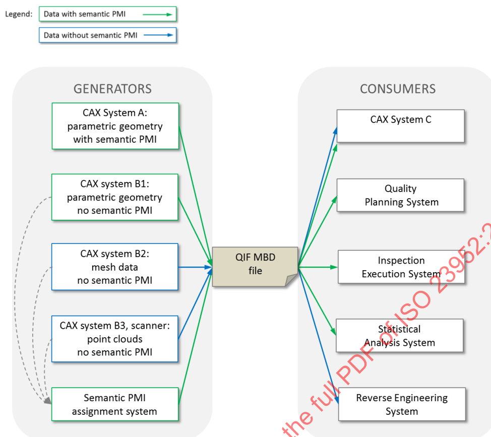
Figure 78 – Workflow of QIF MBD Information
