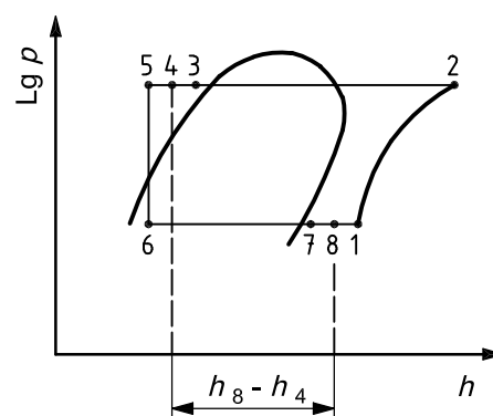
c) Pressure enthalpy diagram showing measuring points
