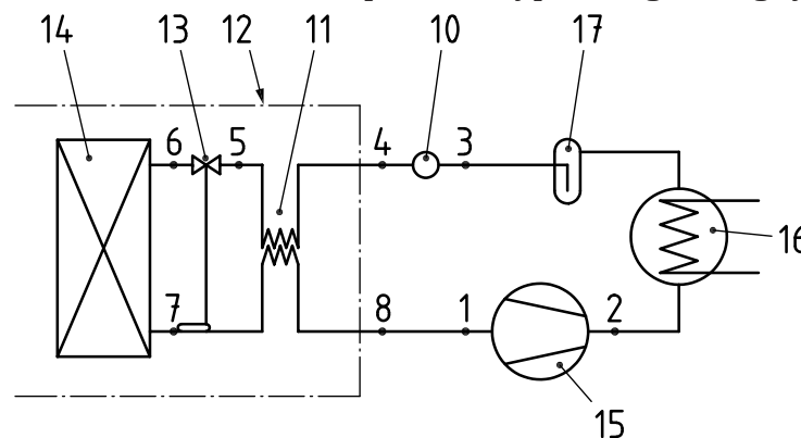
a) Connection to remote compression-type refrigerating system
