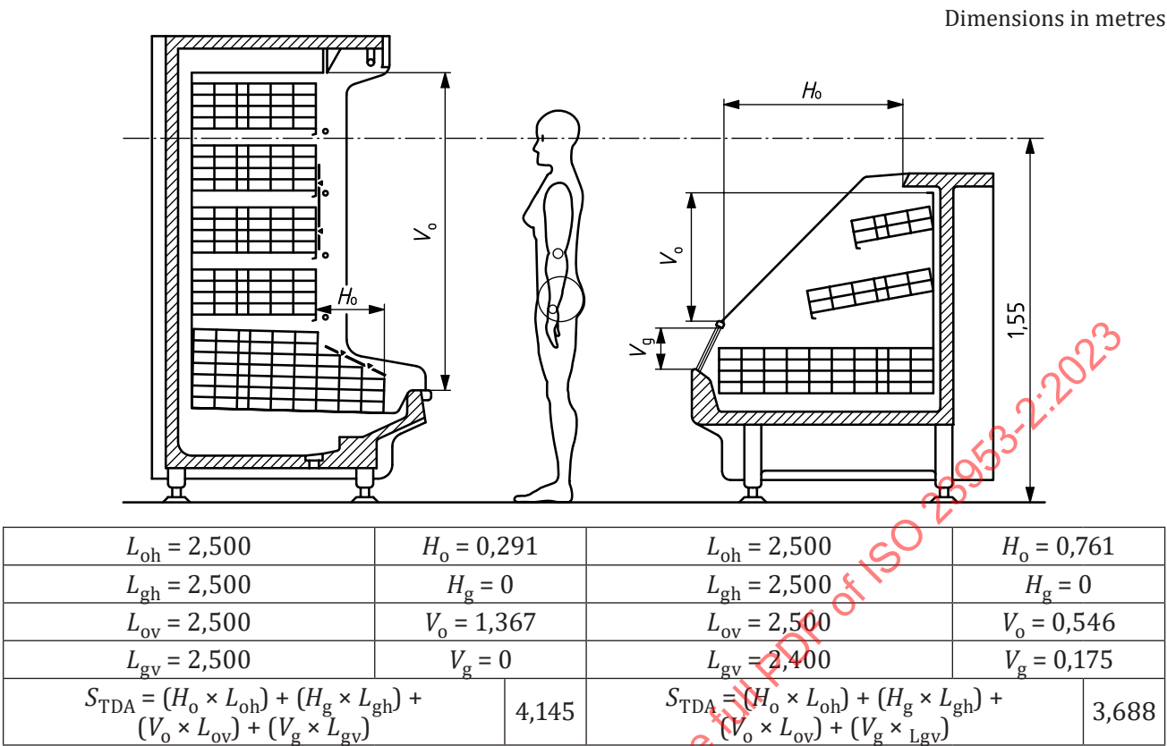
Figure A.4 — Vertical, multi-deck and semi-vertical cabinets
