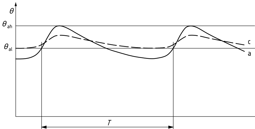
a) Temperature curve with the highest minimum value of all M-package
