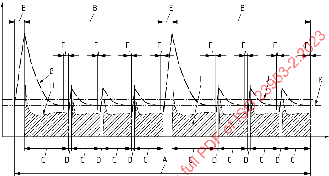
Figure 36 — Refrigeration cycle — Constant evaporating pressure — No cycling
