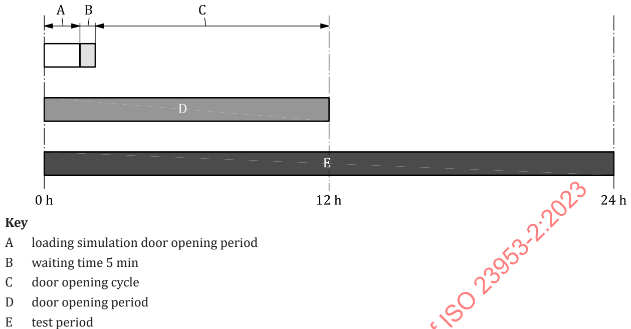
Figure 29 — Door opening schedule
