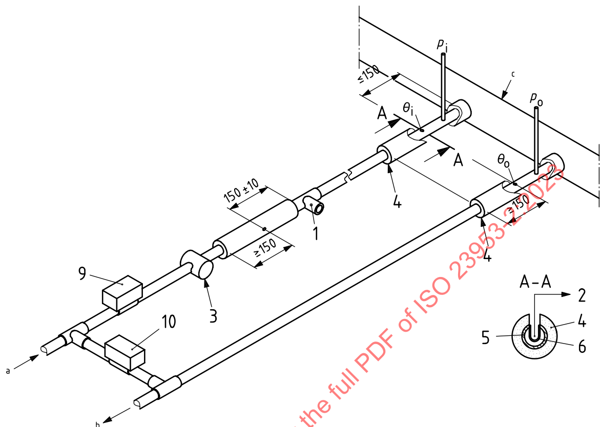
a) Connection to remote indirect-type refrigerating system
