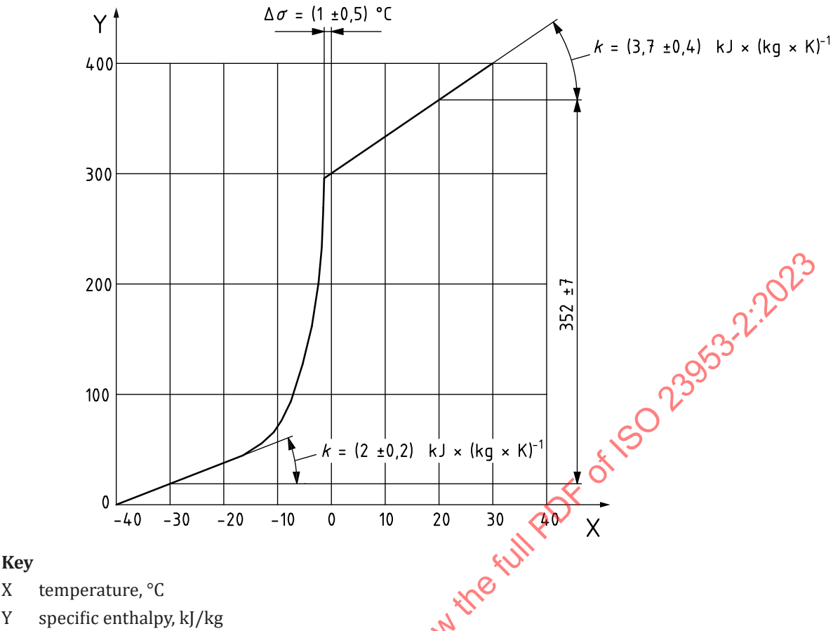
Figure 6 — Thermal characteristics of test packages
