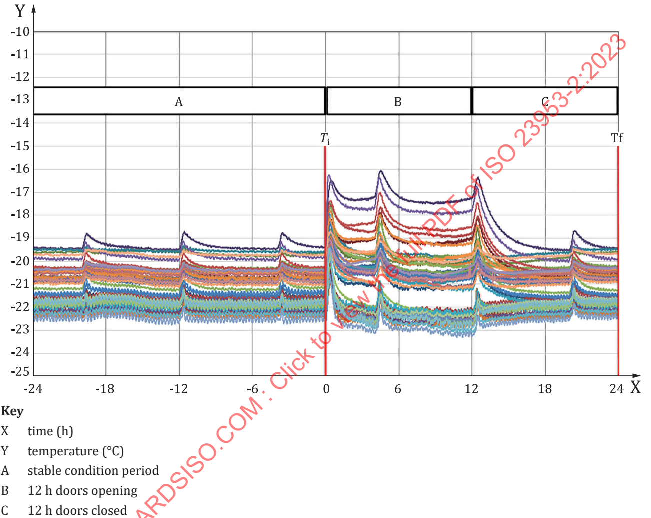
Figure 27 — Example of time temperature diagram showing 24 h test period, ( T_f ) and ( T_i )
