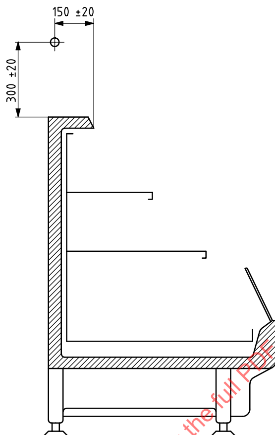
d) Semi-vertical cabinet
