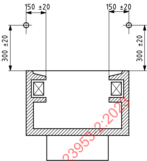
b) Example of horizontal, open, island site cabinet
