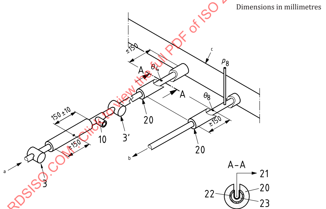
a) Connection to remote compression-type refrigerating system
