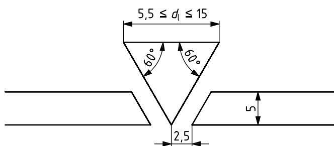
a) Dimensions of load limit line
