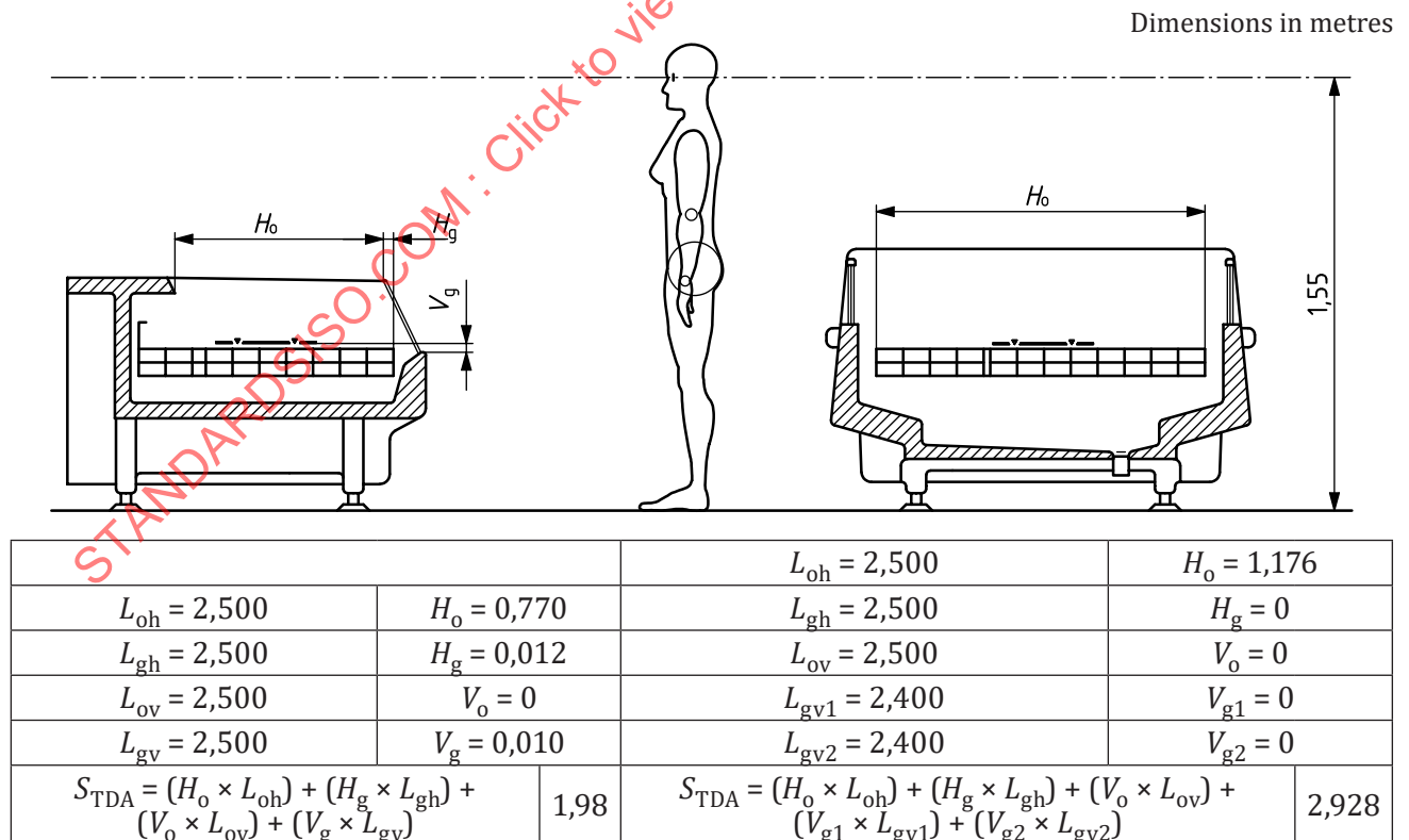
Figure A.3 — Horizontal, open, wall-site and island cabinets with sensitive foodstuff load
