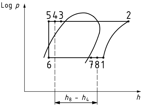
c) Pressure enthalpy diagram showing points referred to in Figure 34 b)
