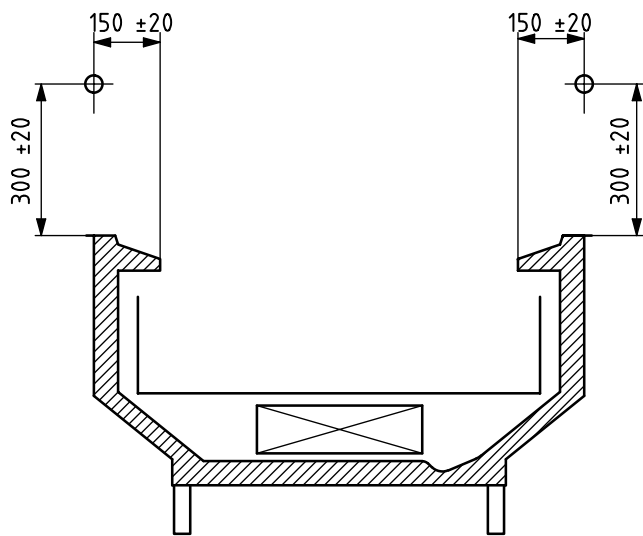
a) Example of horizontal, open, island site cabinet
