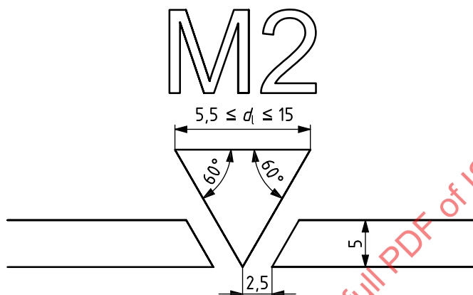
a) Dimensions of load limit line
