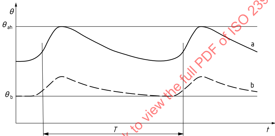
b) Temperature curve of coldest M-package
