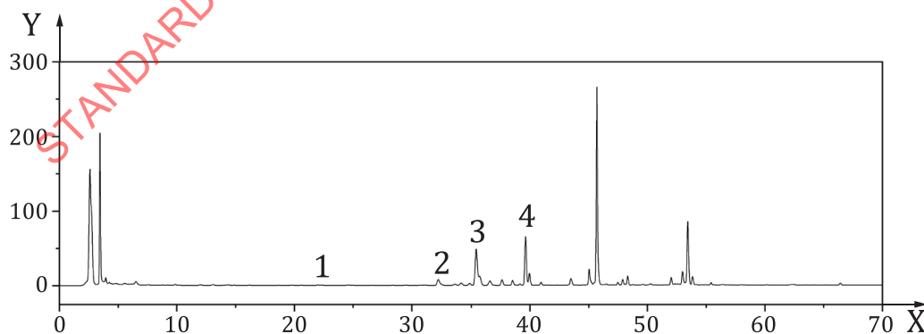
a) Chromatogram of Bupleurum longiradiatum root
