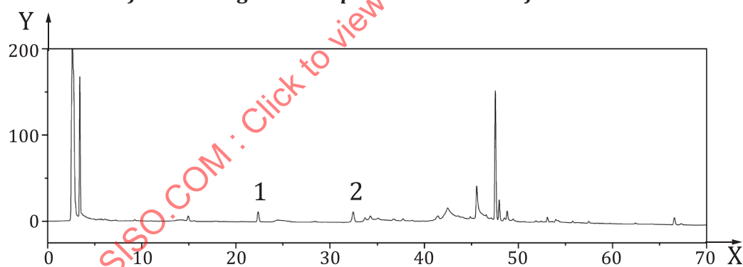
d) Chromatogram of bupleurum falcatum root
