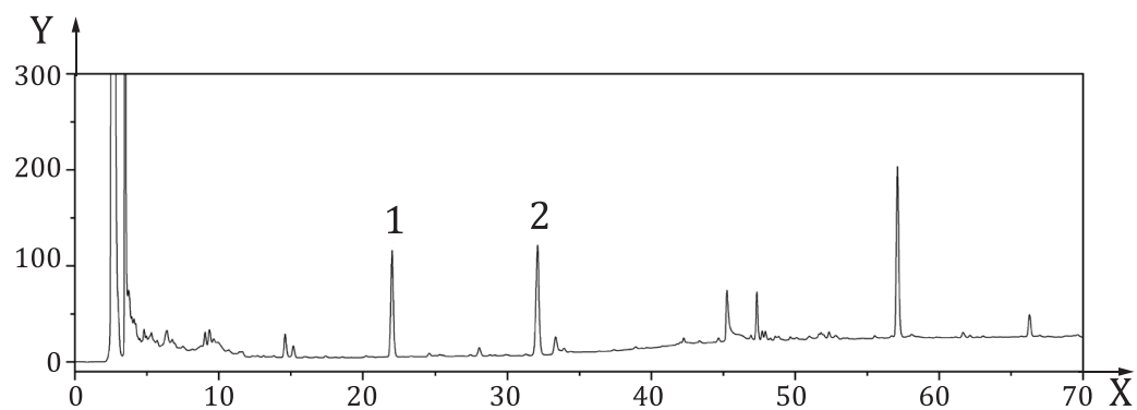
b) Chromatogram of Bupleurum chinense root
