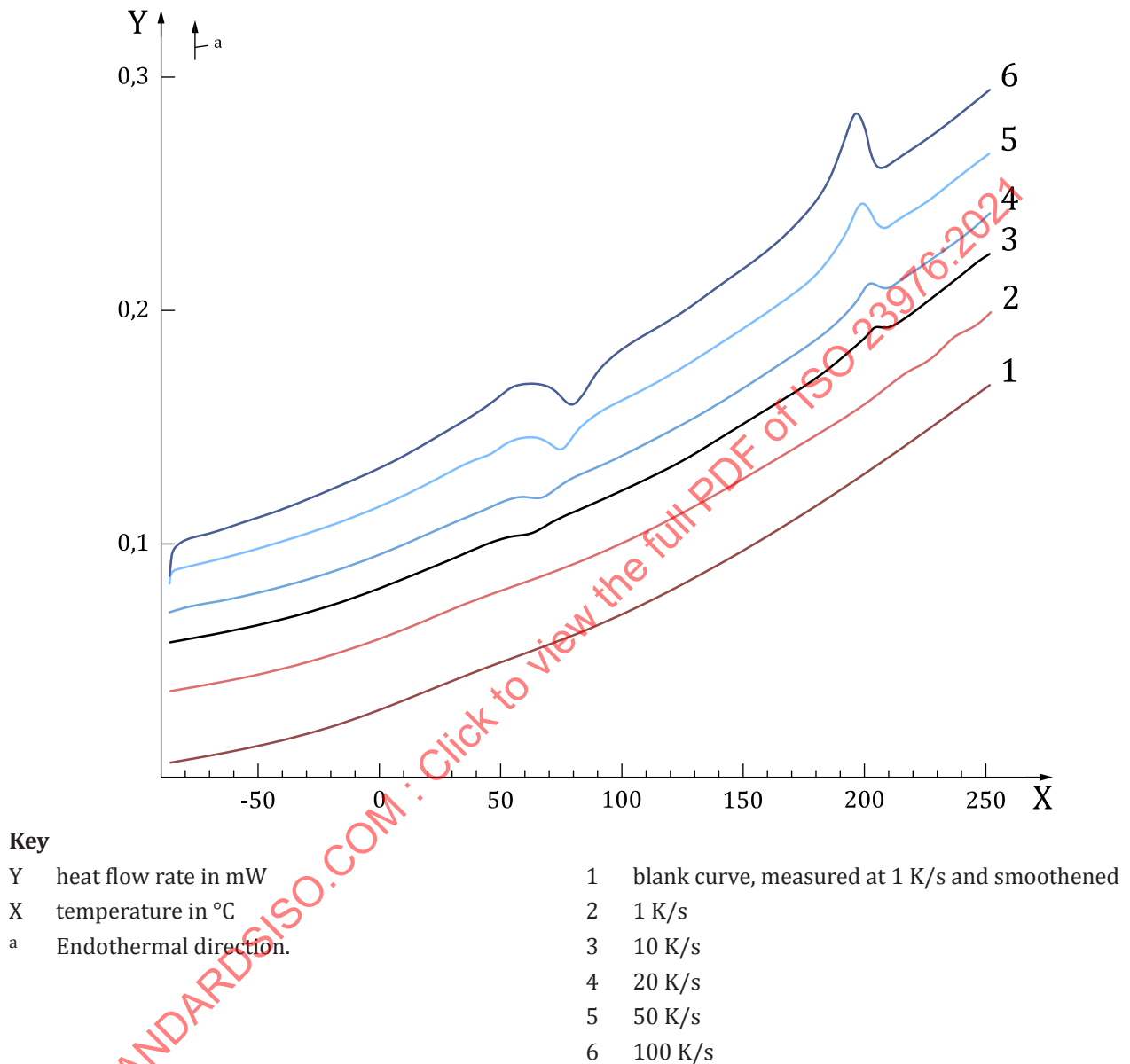
Figure 7 — Heating runs of amorphous PBT at different heating rates [23]
