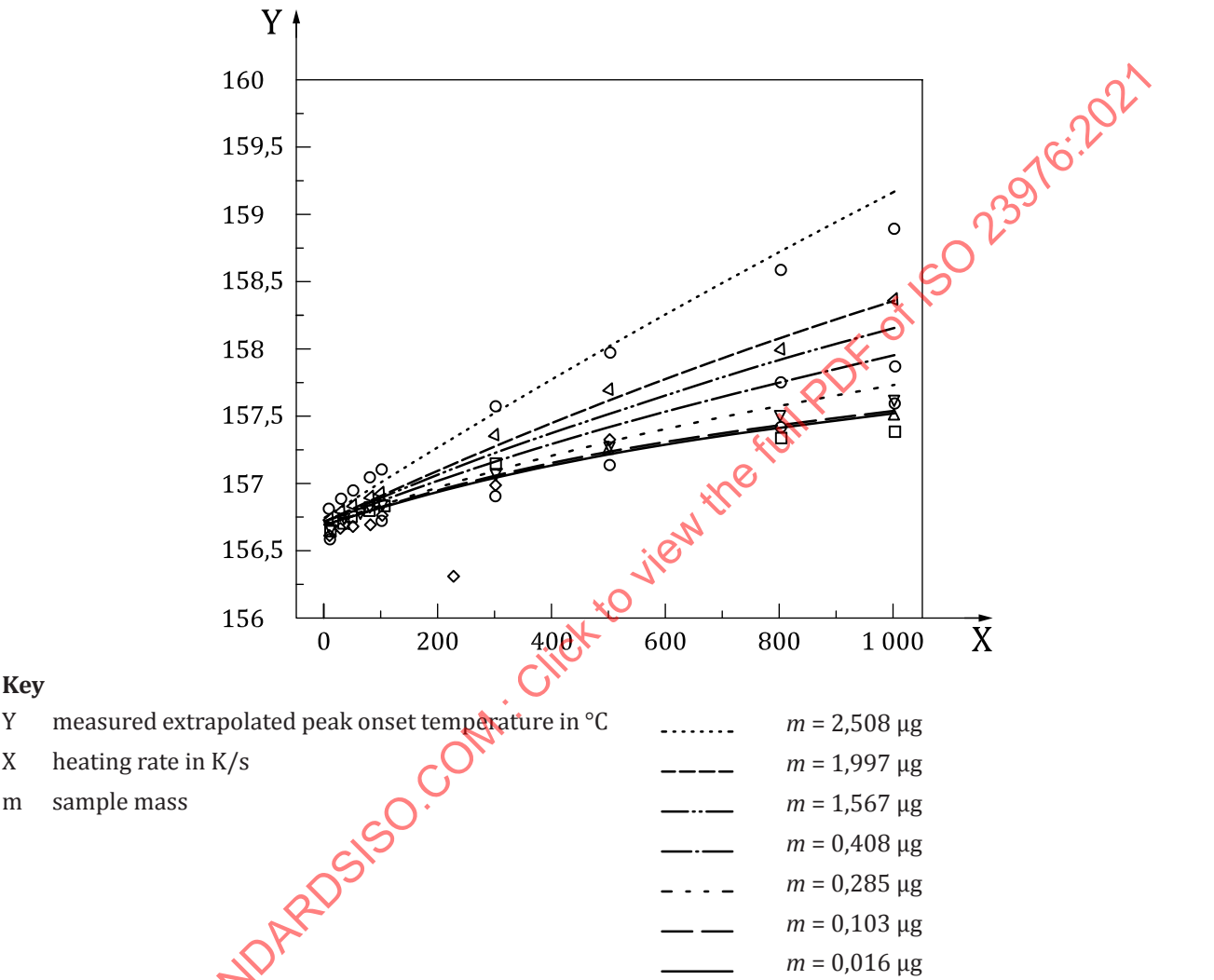
Figure 5 — Extrapolated peak onset temperatures of indium as a function of heating rate and sample mass[14],[17]
