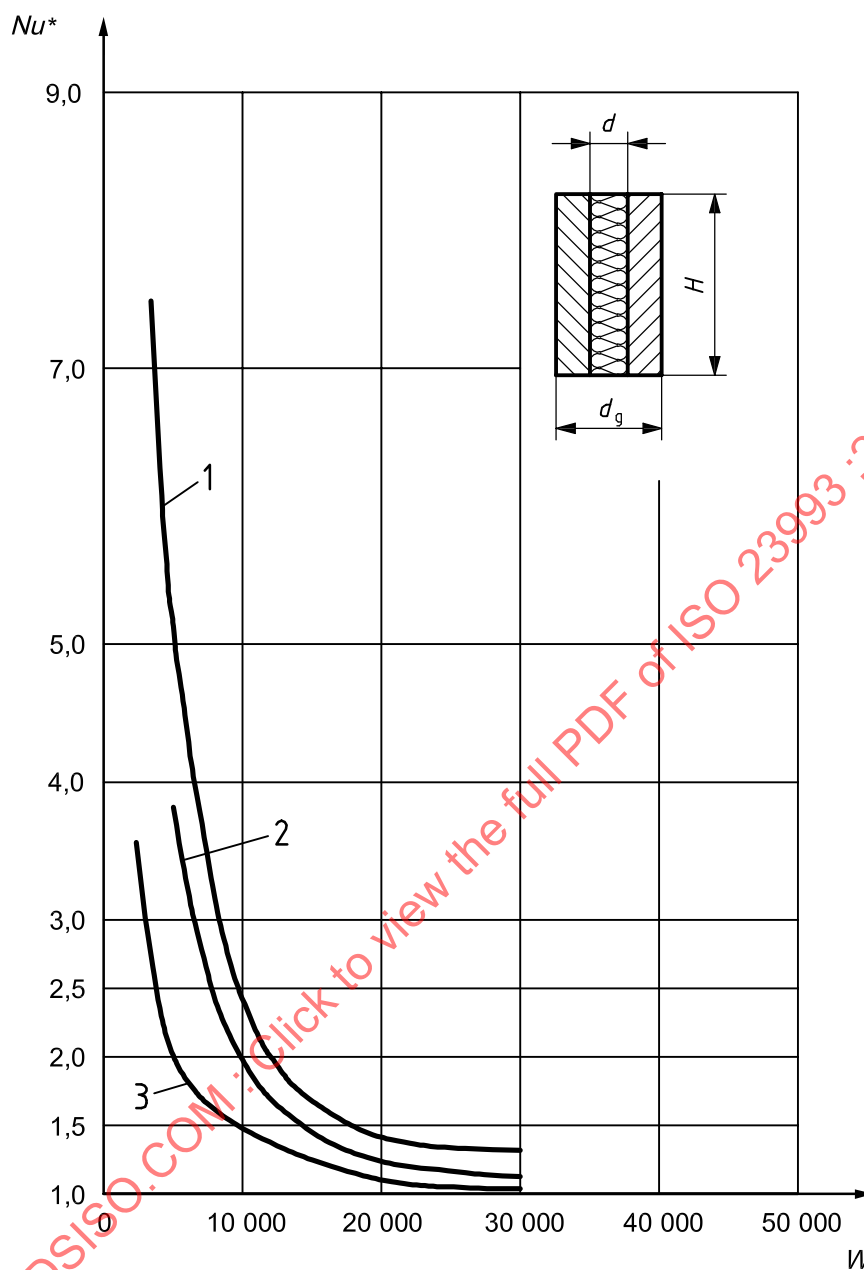
Figure A.6 — Modified Nusselt number for total thickness d_g = 0,60 m of the insulation system
