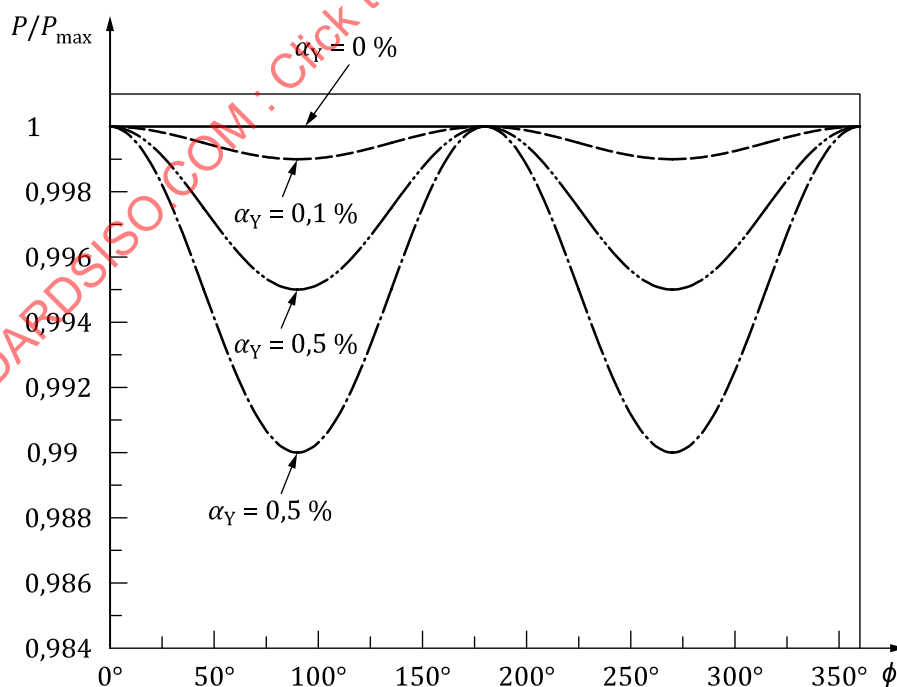
Figure A.3 — Influence of absorptance difference on polarization ellipse
