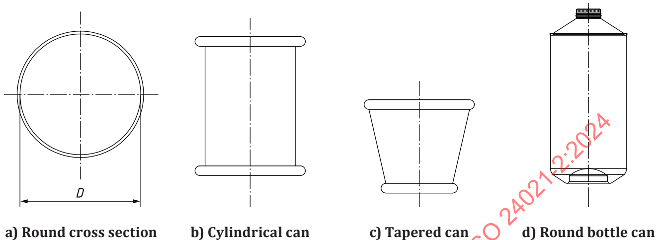
Figure 12 — Round can
