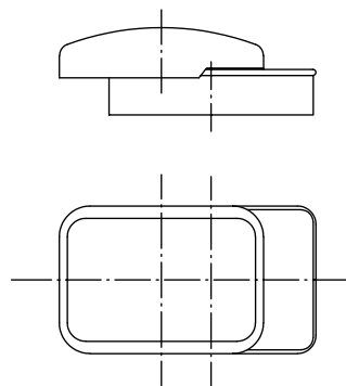
Figure 6 — Slip-lid can
