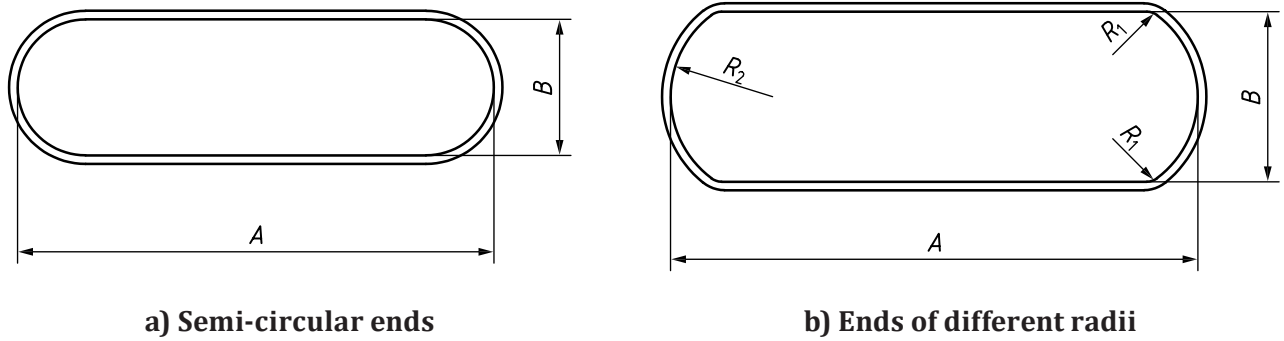
Figure 14 — Obround can
