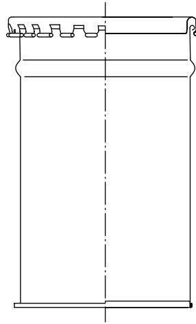
Figure 7 — Crimped-cover can
