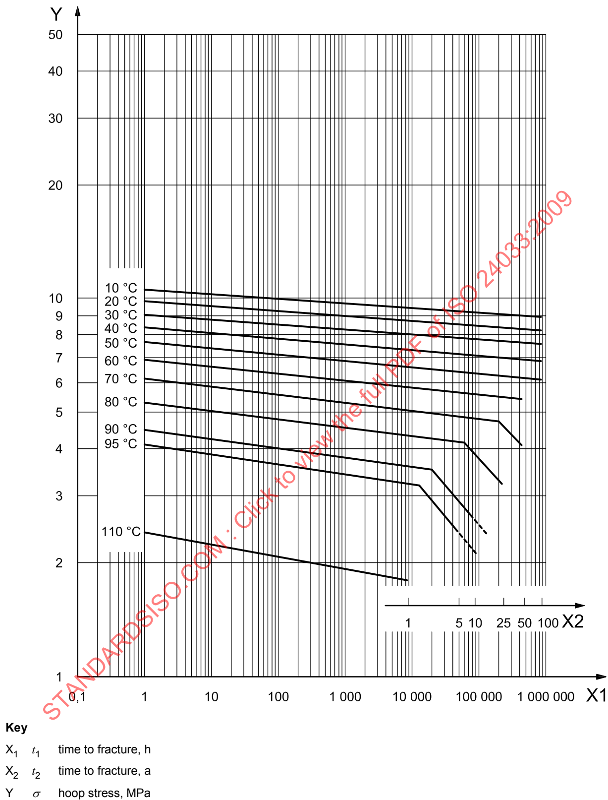
Figure 1 — Expected strength of PE-RT type I pipes
