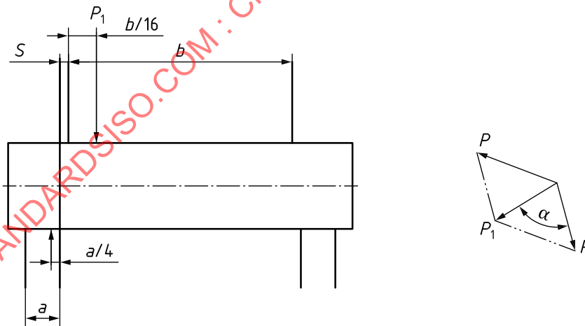
Figure A.4 — Forces and size the of the shaft
