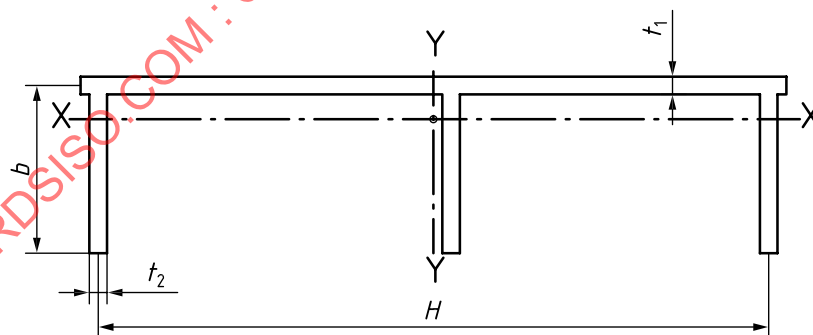
Figure A.3 — Size of the support, Z-Z section
