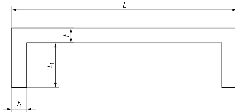
Figure A.2 — Shear surface of the lever support
