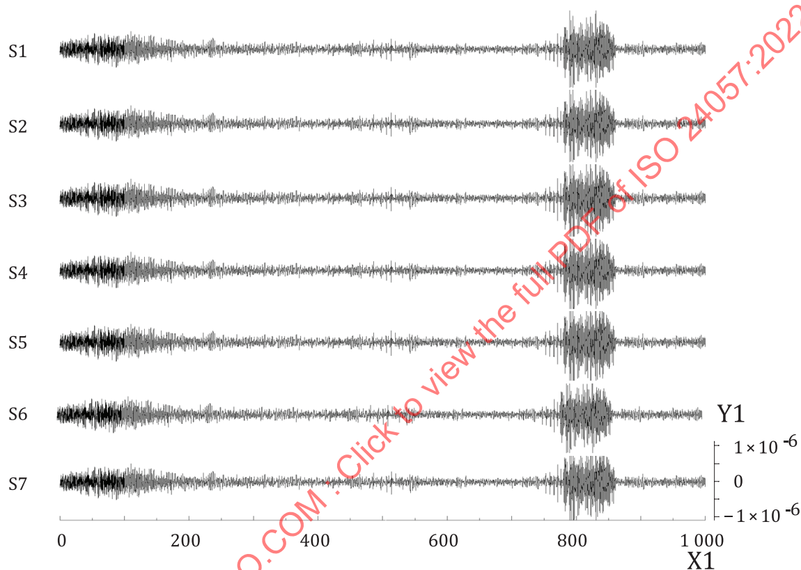
a) Vertical component of microtremor records measured in the double concentric equilateral triangle array by seven sensors
