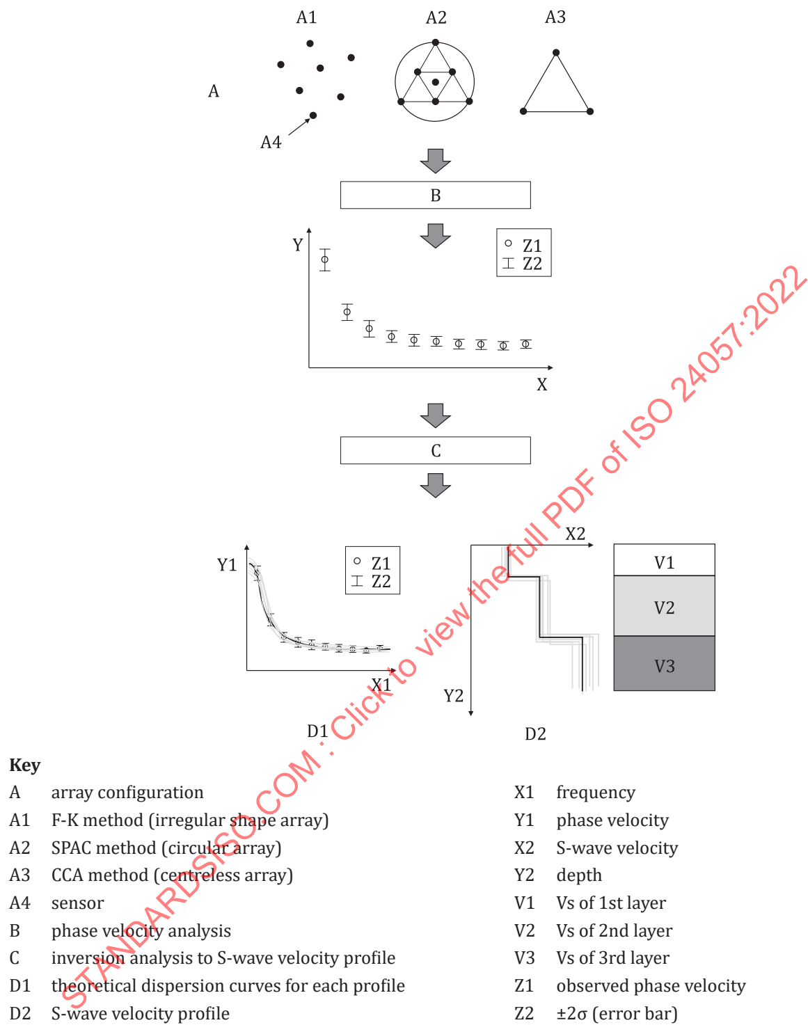
Figure 4 — Flow chart of the data analysis of array measurement of microtremors
