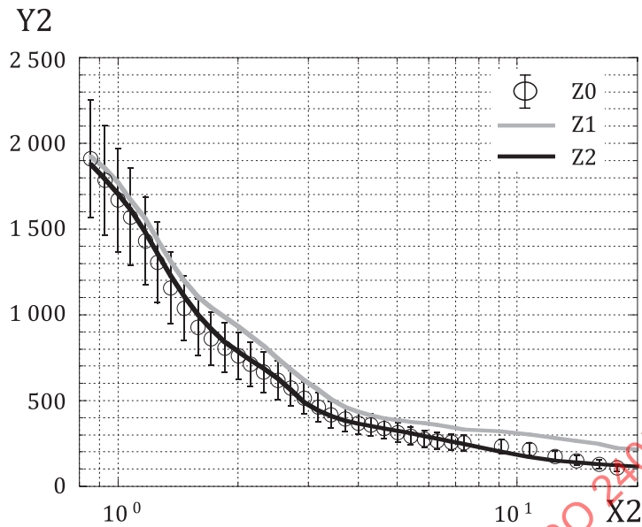
b) Dispersive characteristics (dispersion curve) of the microtremors
