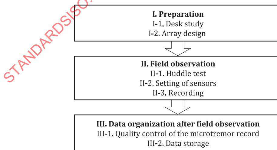
Figure 3 — Typical flow chart of a survey procedure of array measurement of microtremors
