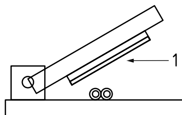
Figure 7 — Test set up for Guillotine test
