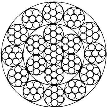
with steel core (WS)
