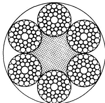
with fibre core (FC)
