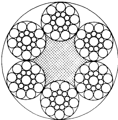
with fibre core (FC)
