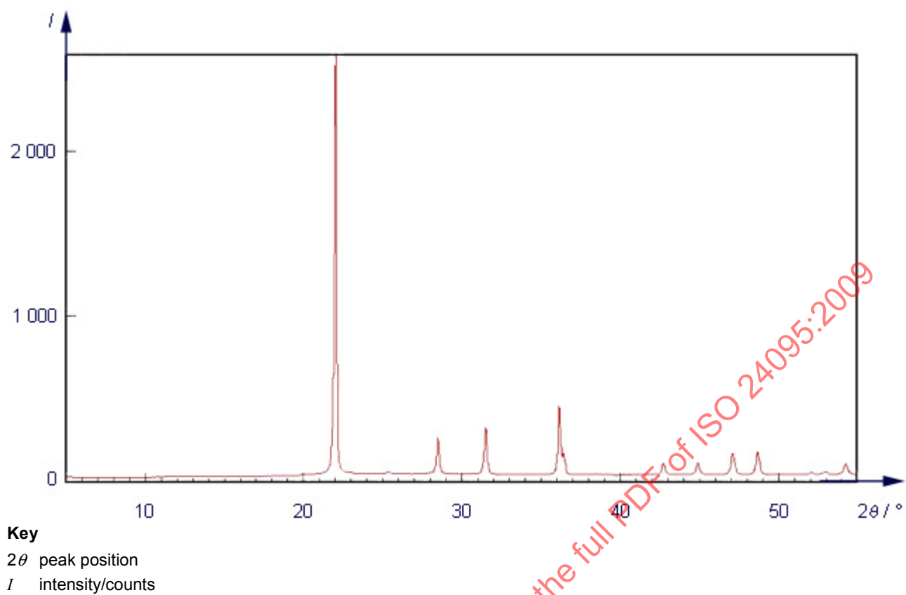
Figure B.1 — An X-ray diffraction scan of crystalline \alpha -cristobalite
