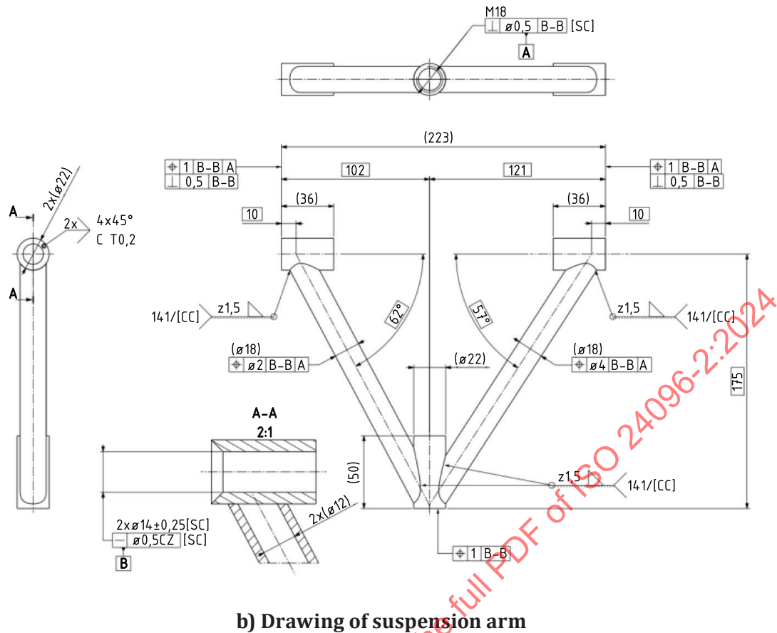
Figure A.3 — TPD of upper arm in front suspension with requirement classification
