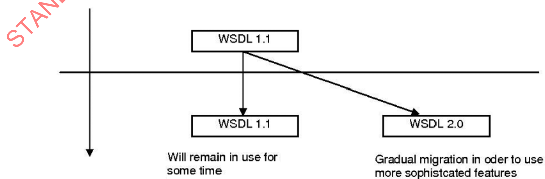
Figure 8 — WSDL migration
