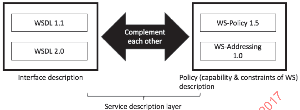
Figure 4 — WSDL, WS-Policy, and WS-Addressing relationship
