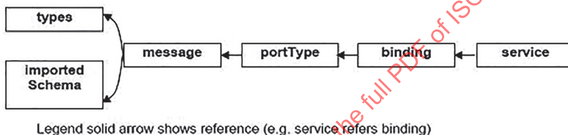
Figure A.2 — WSDL 1.1 structure
