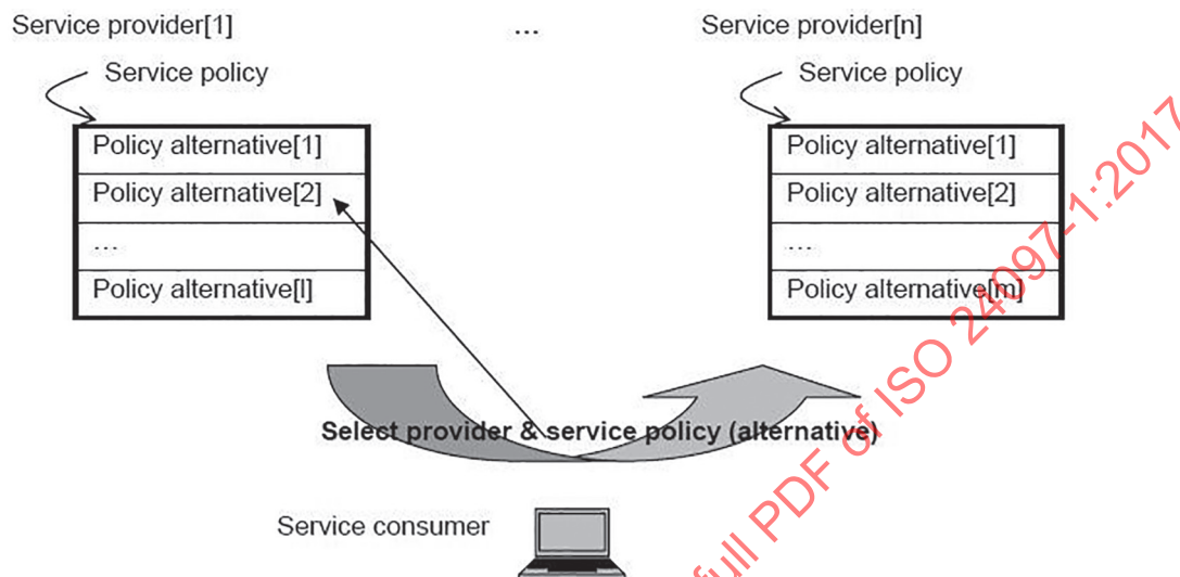
Figure 10 — Service provider and policy alternative selection
