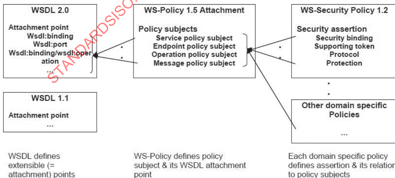
Figure 11 — WSDL, WS-Policy, and domain specific policy
