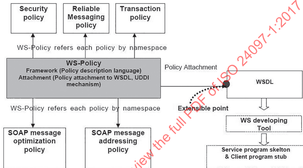
Figure 9 — WS-Policy structure
