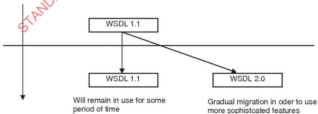
Figure 8 — WSDL migration
