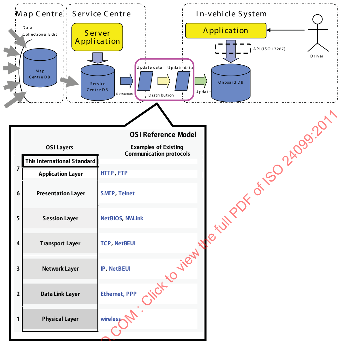
Figure 2 — Reference architecture
