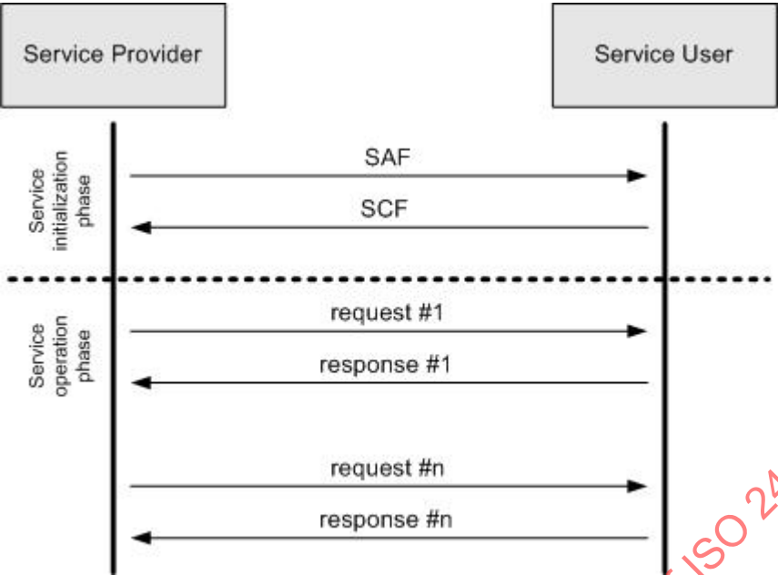
Figure 4 — Service provision with SCF
