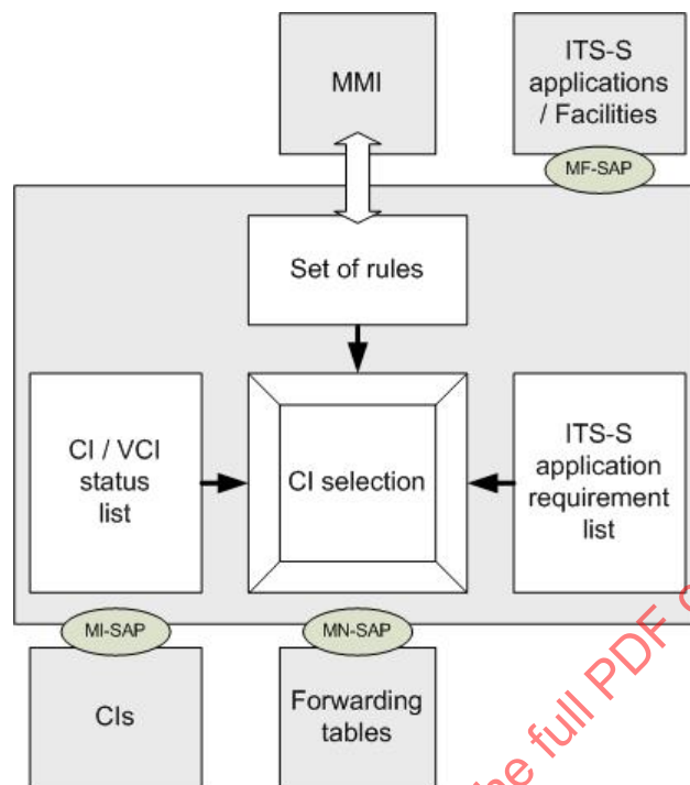
Figure 8 — CI selection management
