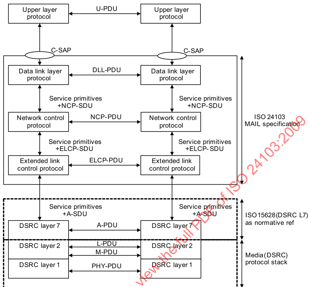
Figure 5 — Overview of DSRC and MAIL service interfaces and protocols
