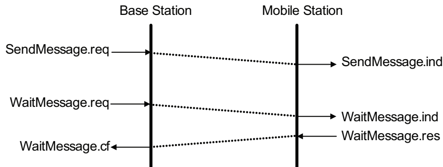
Figure 7 — Logical relationships between sub-primitives defined in ACTION service
