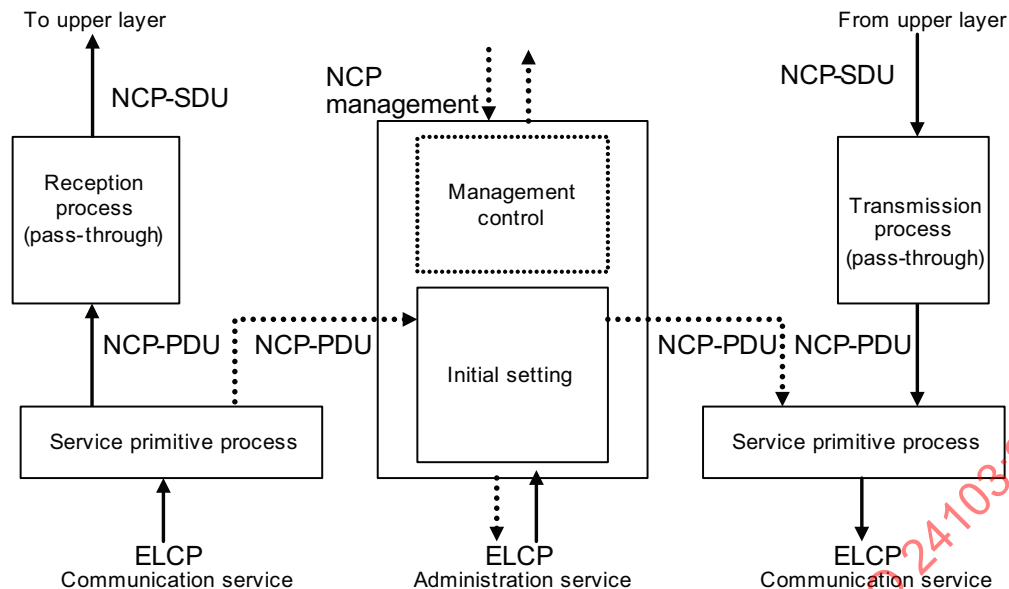
Figure 10 — NCP configuration
