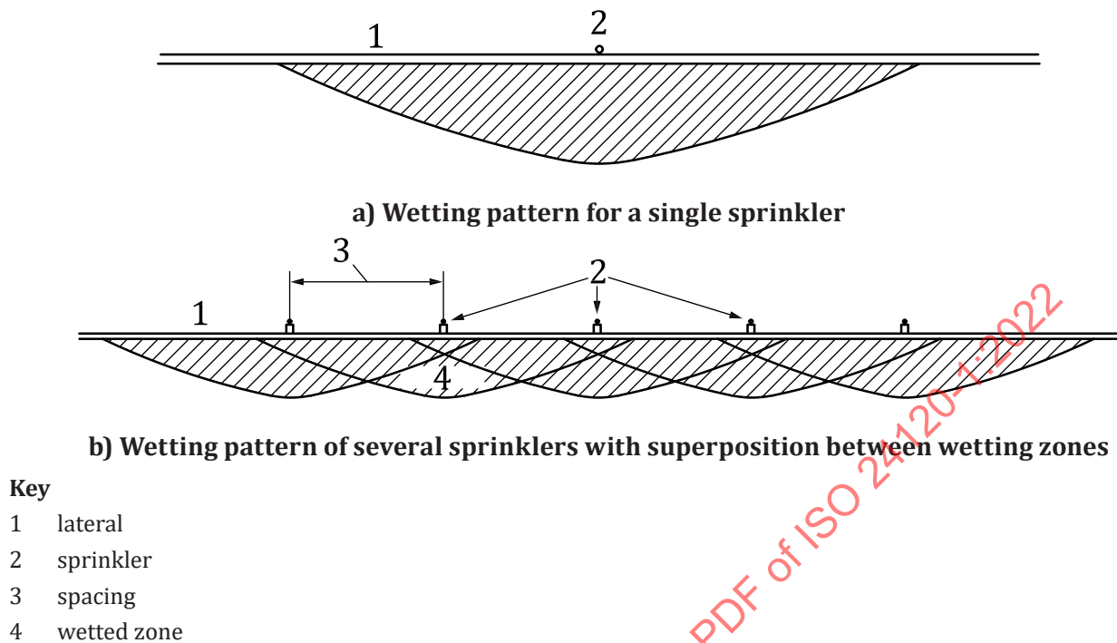
Figure 2 — Sprinkler irrigation [1]
