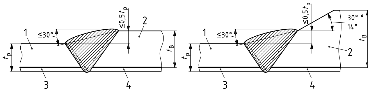
b) the matching pipe is CRA clad or lined steel pipe
