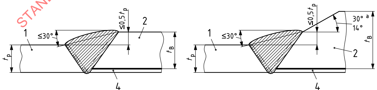
a) the matching pipe is CRA solid pipe
