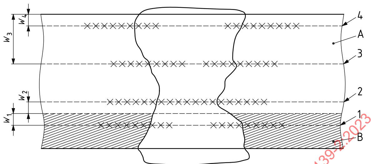
a) welded clad fitting
