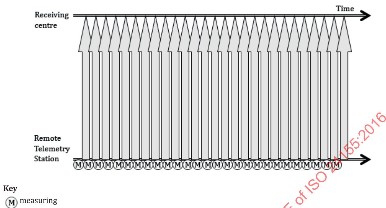
Figure E.3 — Continuous transmission
