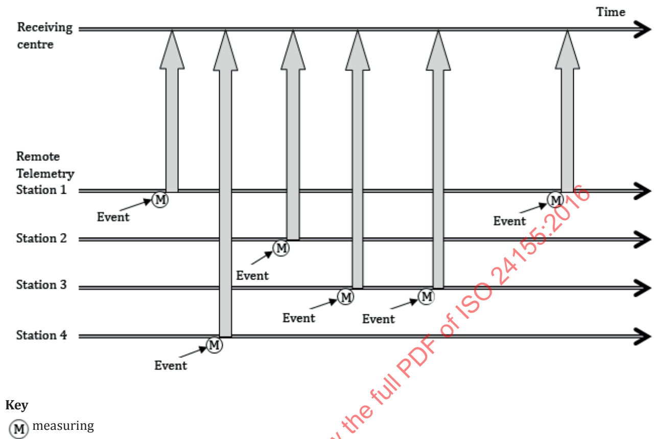
Figure E.6 — Event reporting
