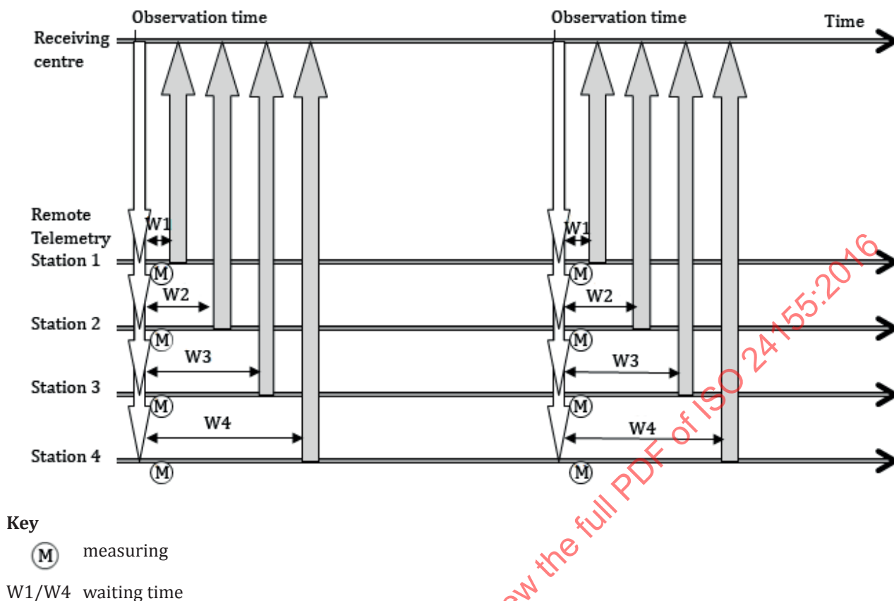
Figure E.5 — Batch polling and sequential reporting
