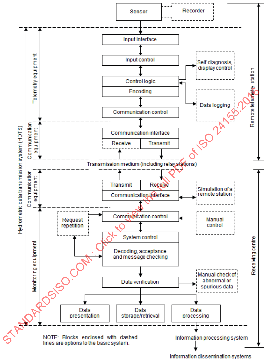
Figure B.1 — Functional block diagram of hydrometric data transmission systems
