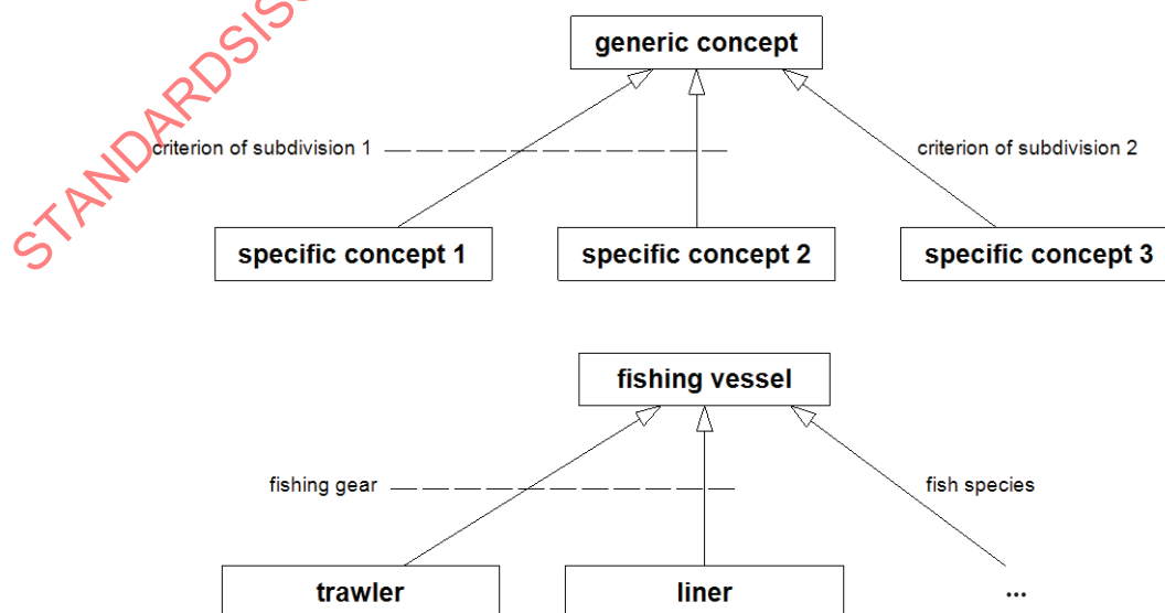
Figure 5 — Criterion of subdivision: ISO 704 > ISO 24156-1 user-defined UML profile
