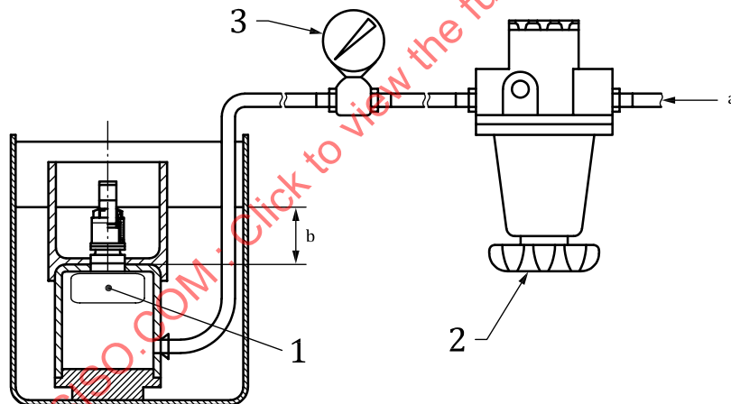
Figure 2 — Valve core leakage test set-up
