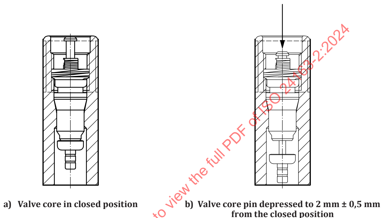
Figure 5 — Valve core air flow rate position
