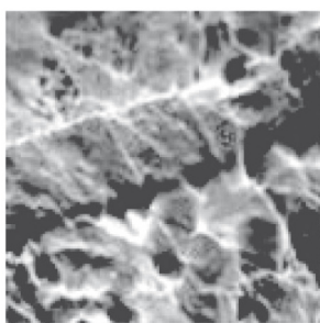
Figure B.3 — Effect of ion milling on titanium [back-scattered electron (BSE) images]
