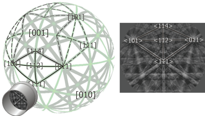
Figure 12 — Schematic diagram showing how a calibration EBSD (right, with a “kite” labelled) can be misinterpreted when used to calibrate an EBSD detector. There are several possible viewpoints for the EBSD detector that would produce the same EBSD (as shown by labelled “kites” on the left). Miscalibration of this kind will result in consistently rotated, incorrect orientation data.
