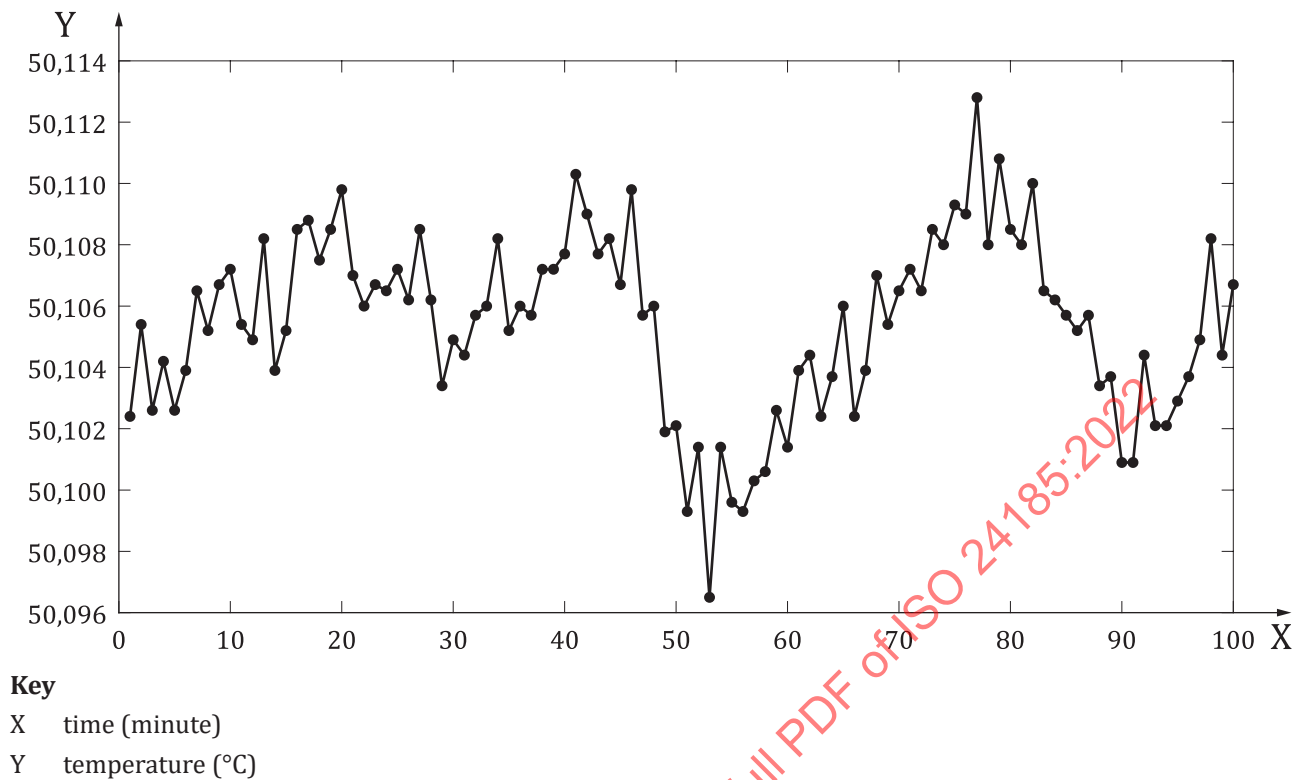
Figure A.3 — Time series of temperature readings
