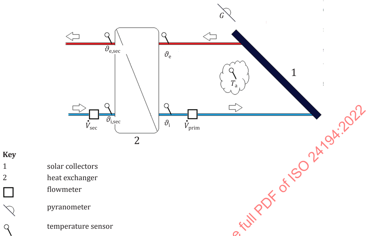
Figure 6 — Schematic drawing showing the measurement points. System with heat exchanger (Source: PlanEnerg)
