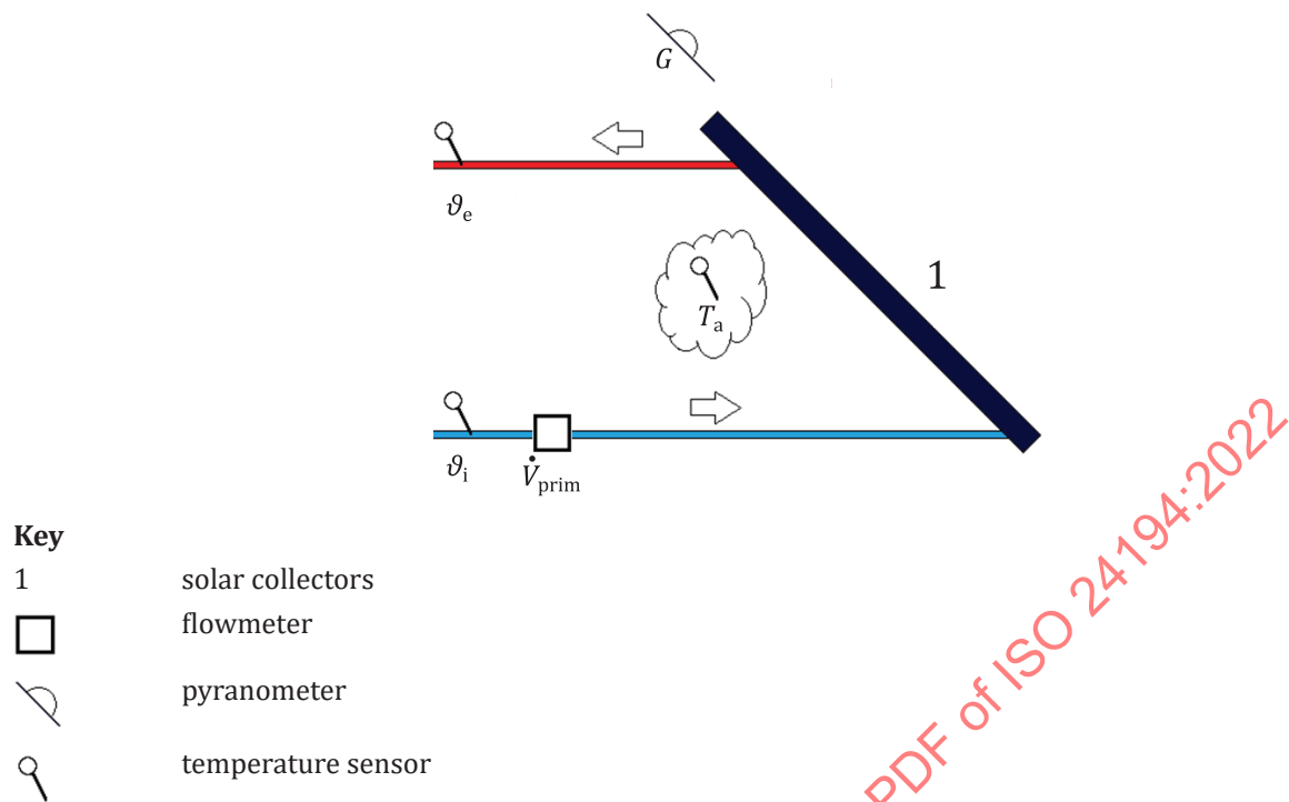
Figure 5 — Schematic drawing showing the measurement points. System without heat exchanger (Source: PlanEnergi)
