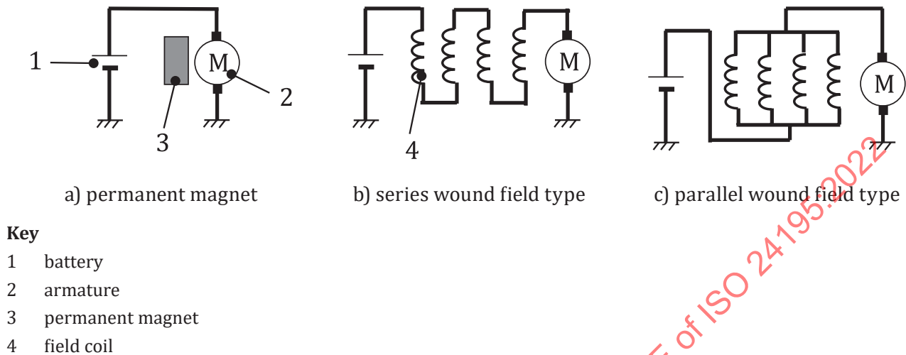
Figure 3 — Magnetic field types
