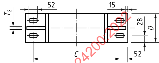
i) Design for clamp 'type B' for pipe NPS 10
