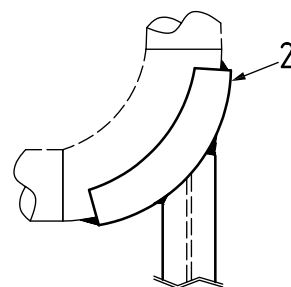
h) Elbow stanchion weld detail (H section type B)
