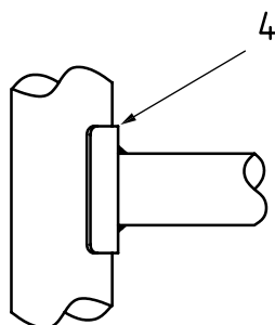
c) Pipe trunnion weld detail (pipe section)
