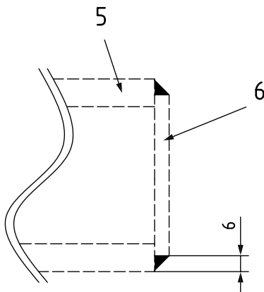
i) Detail for end cap (pipe section)
