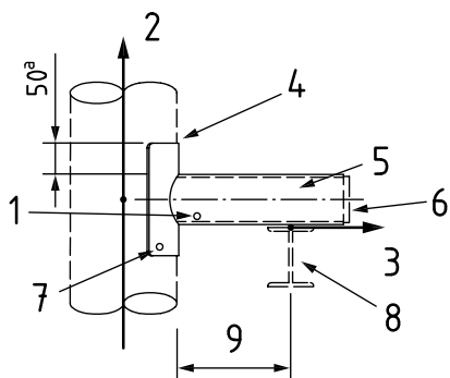
a) Pipe trunnion - pipe/beam section
