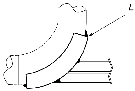
h) Elbow trunnion weld detail (H section Type B)
