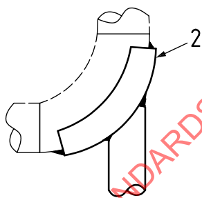
f) Elbow stanchion weld detail (pipe section)
