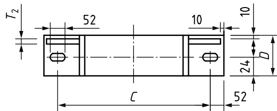
h) Design for clamp 'type B' for pipe NPS 3 to NPS 8
