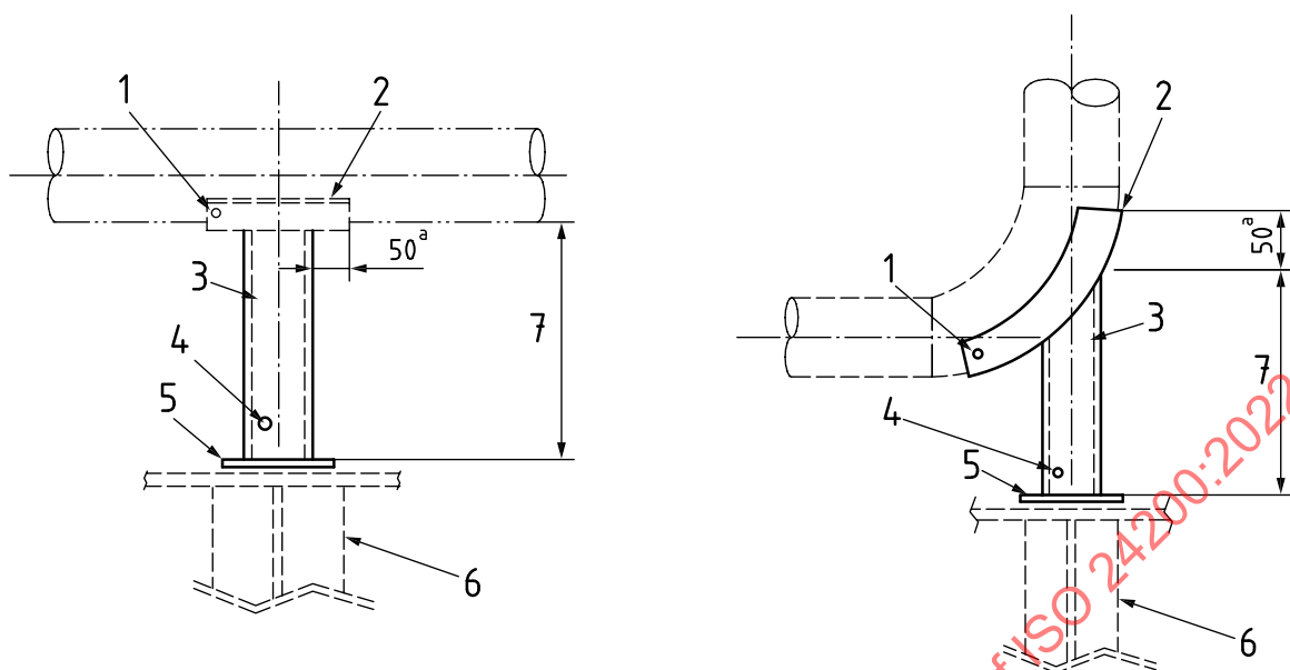
a) Pipe stanchion – pipe/beam section
