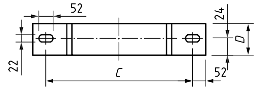
g) Design for clamp 'type B' for pipe NPS 3/4 to NPS 2
