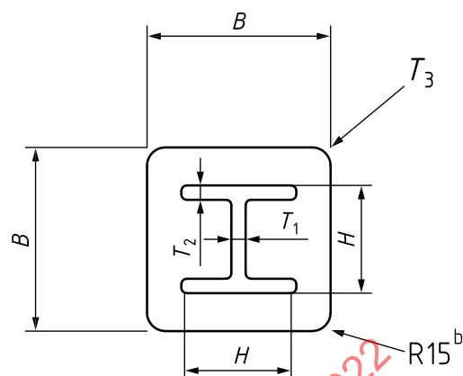
j) Detail for base plate (H section type A or type B)
