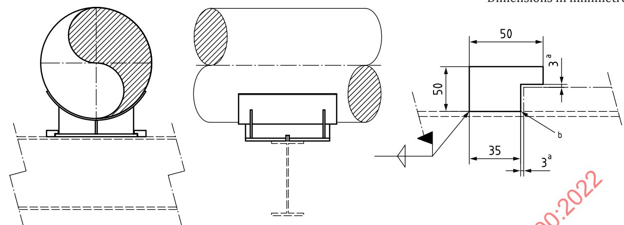
a) Guide and hold-down support type A
