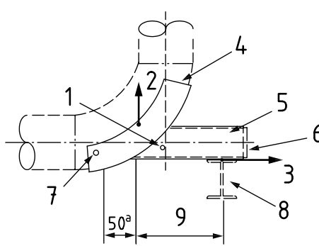
b) Elbow trunnion - pipe/beam section
