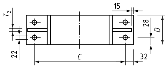
f) Design for clamp 'type A' for pipe NPS 10
