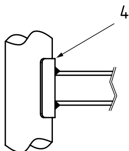
d) Pipe trunnion weld detail (H section Type A)
