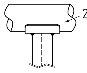
e) Pipe stanchion weld detail (H section type B)
