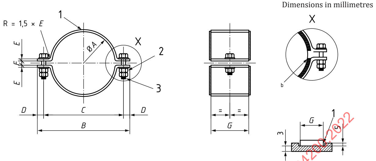
a) Clamp detail (typical)
