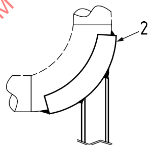
g) Elbow stanchion weld detail (H section type A)
