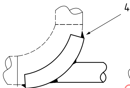
f) Elbow trunnion weld detail (pipe section)
