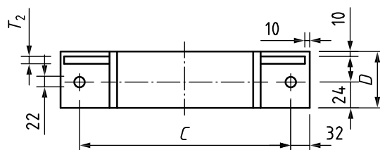
e) Design for clamp 'type A' for pipe NPS 3 to NPS 8
