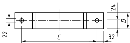
b) Design for isolation pad for pipe NPS \frac{3}{4} to NPS 8
