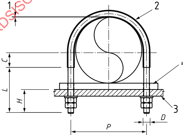
a) Overall design
