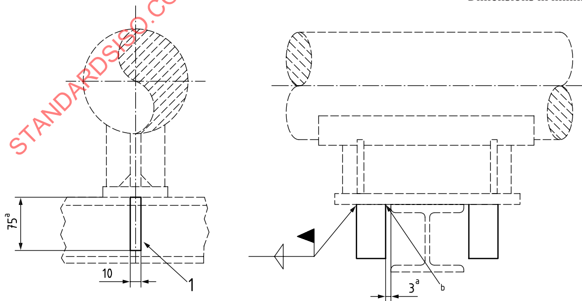
a) Line-stop support type A
