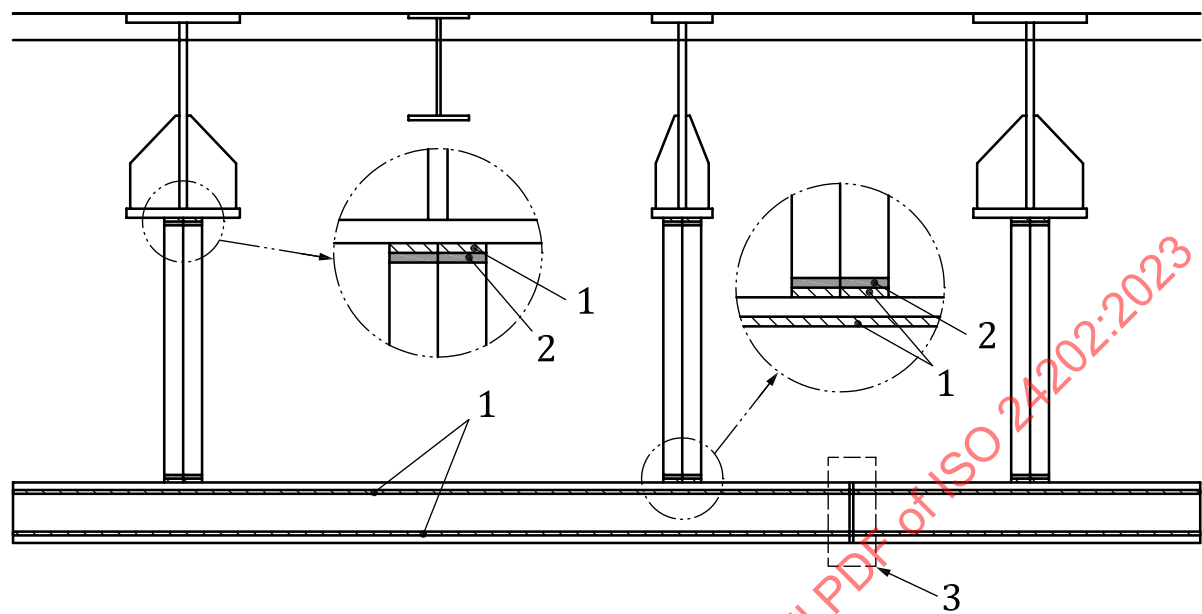
a) Inspection requirements for monorail beams including supporting structures
