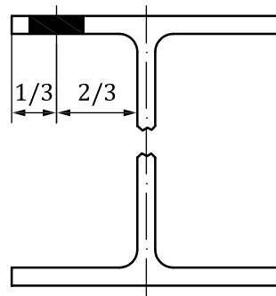
Figure A.2 — Location of test specimens from H-beams
