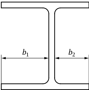
Figure A.5 — Web off centre tolerance of H-beam
