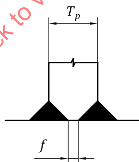
b) Partial joint penetration welding
