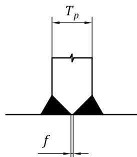
c) Complete joint penetration welding
