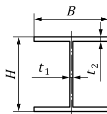
Figure A.3 — Dimension of H-beams
