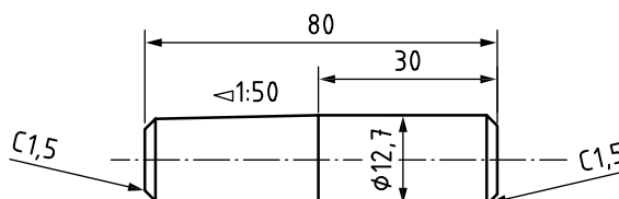
Figure C.1 — Example size of stud
