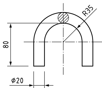
Figure B.1 — lifting lug of manifold
