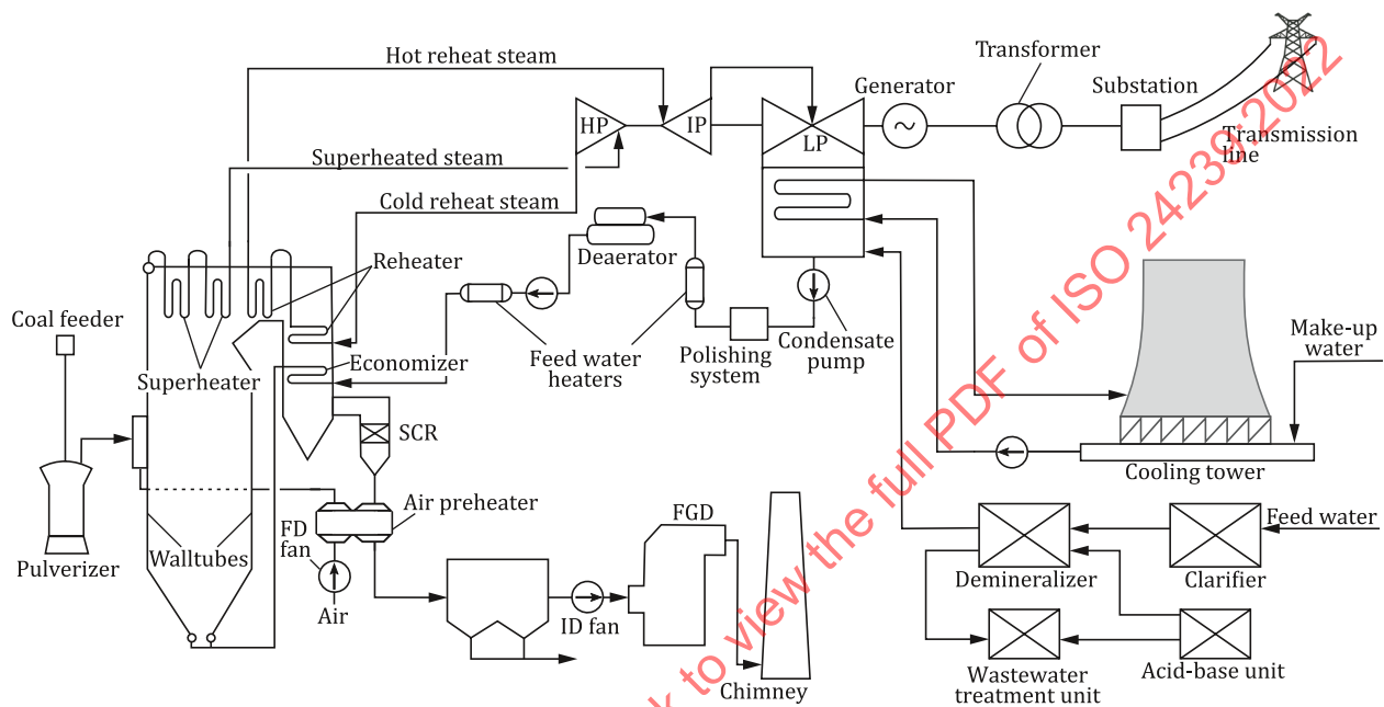
Figure A.1 — Example of a fossil fuel power plant
