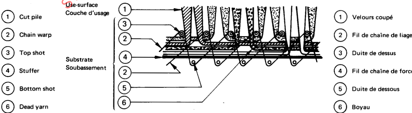
FIGURE 3 — Jacquard weave carpet, two-shot (warpways section)
