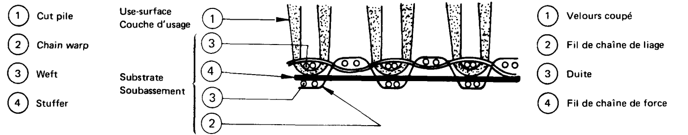
FIGURE 9 – Gripper Axminster carpet (warps section)
