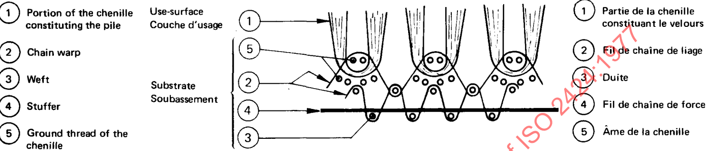
FIGURE 7 – Chenille Axminster carpet (warps section)
