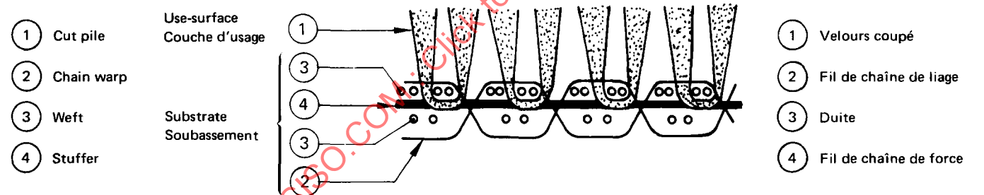
FIGURE 8 – Spool Axminster carpet (warps section)
