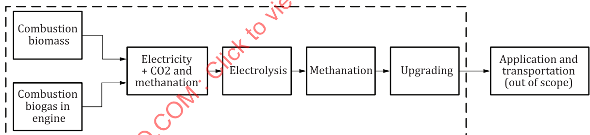
Figure A.3 — Scope of standard schematic overview: Power to gas from biomass source process
