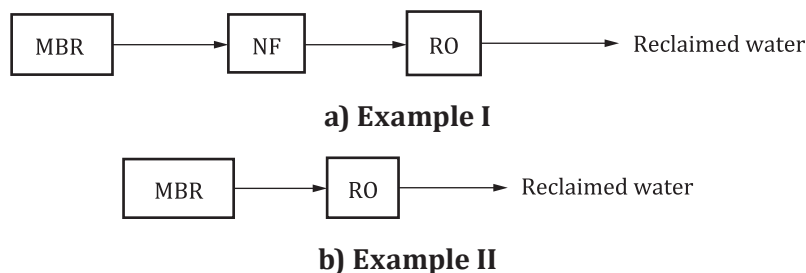
Figure 6 — Typical examples of combined process for advanced treatment
