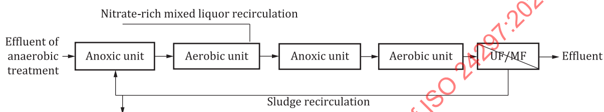
Figure 5 — Flow chart of a typical two-stage A/O process with sidestream MBR
