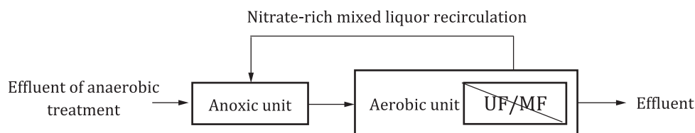
Figure 4 — Flow chart of a typical A/O process with submerged MBR
