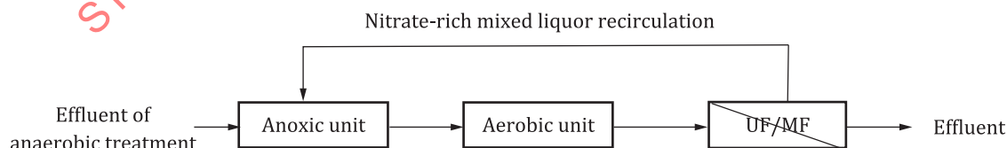
Figure 3 — Flow chart of a typical A/O process with sidestream MBR
