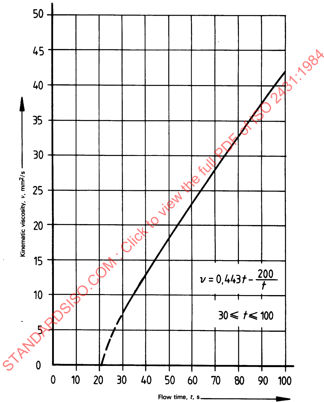
Figure 2 — Calibration curve for 3 mm cup
