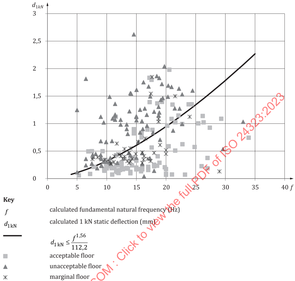
Figure A.2 — Baseline design criteria derived from combined German and Canadian databases
