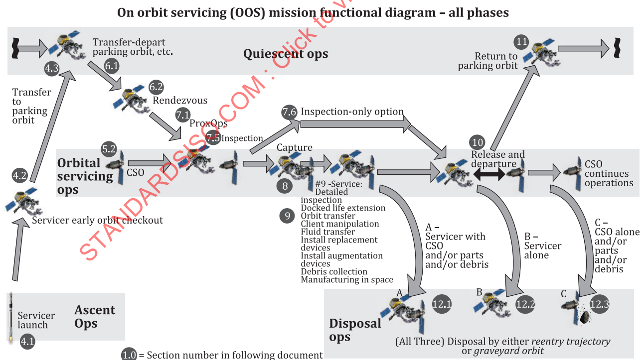
Figure B.1 — On-orbit servicing (OOS) mission functional diagram
