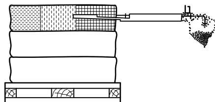
Figure B.10 — Cone-shaped sampling device
