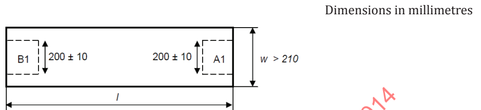
Figure 2 — Cutting of panels for short side testing ( w < 100 mm)
